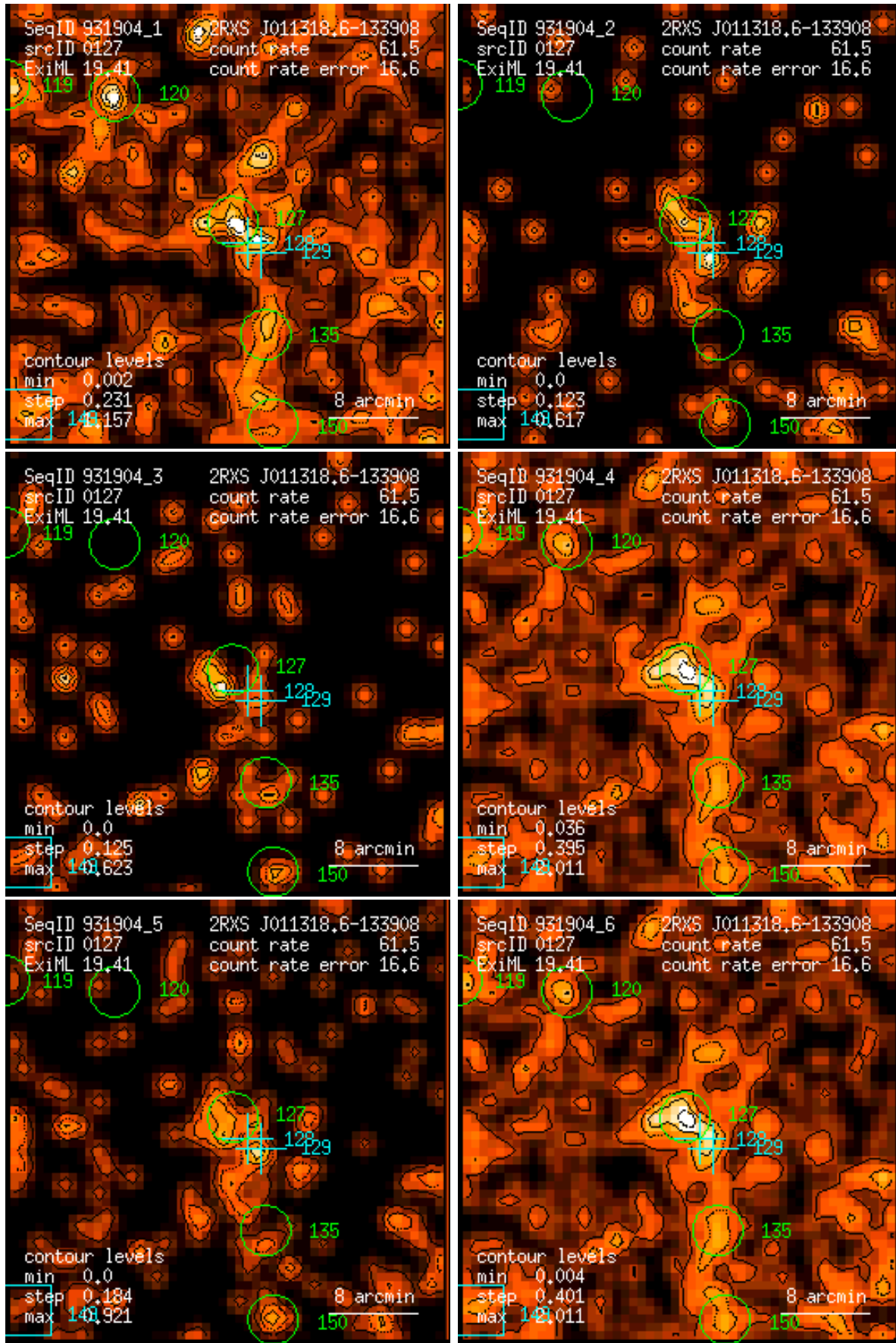
Figure 127: RASS 931904: detection 0127: band rate images, Gaussian filter: (1) PSPC channels 11 – 41, (2) 52 – 90, (3) 91 – 201, (4) 11 – 235, (5) 52 – 201, (6) 11 – 201. Broad band rates in counts/ks. Band rate contour levels in counts/ks/arcmin 2 .
