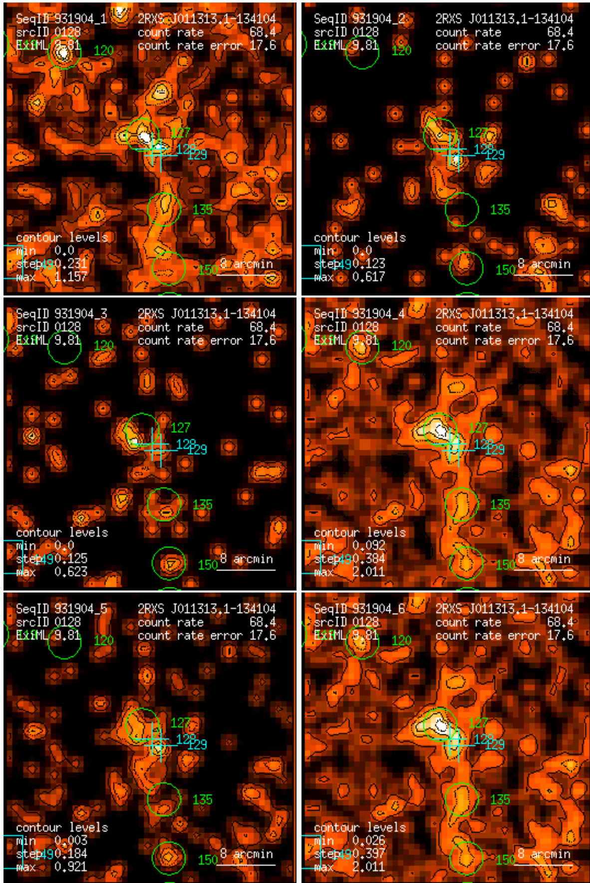
Figure 128: RASS 931904: detection 0128: band rate images, Gaussian filter: (1) PSPC channels 11 – 41, (2) 52 – 90, (3) 91 – 201, (4) 11 – 235, (5) 52 – 201, (6) 11 – 201. Broad band rates in counts/ks. Band rate contour levels in counts/ks/arcmin 2 .
