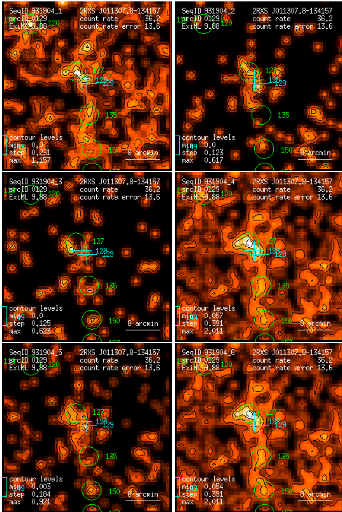
Figure 129: RASS 931904: detection 0129: band rate images, Gaussian filter: (1) PSPC channels 11 – 41, (2) 52 – 90, (3) 91 – 201, (4) 11 – 235, (5) 52 – 201, (6) 11 – 201. Broad band rates in counts/ks. Band rate contour levels in counts/ks/arcmin 2 .
