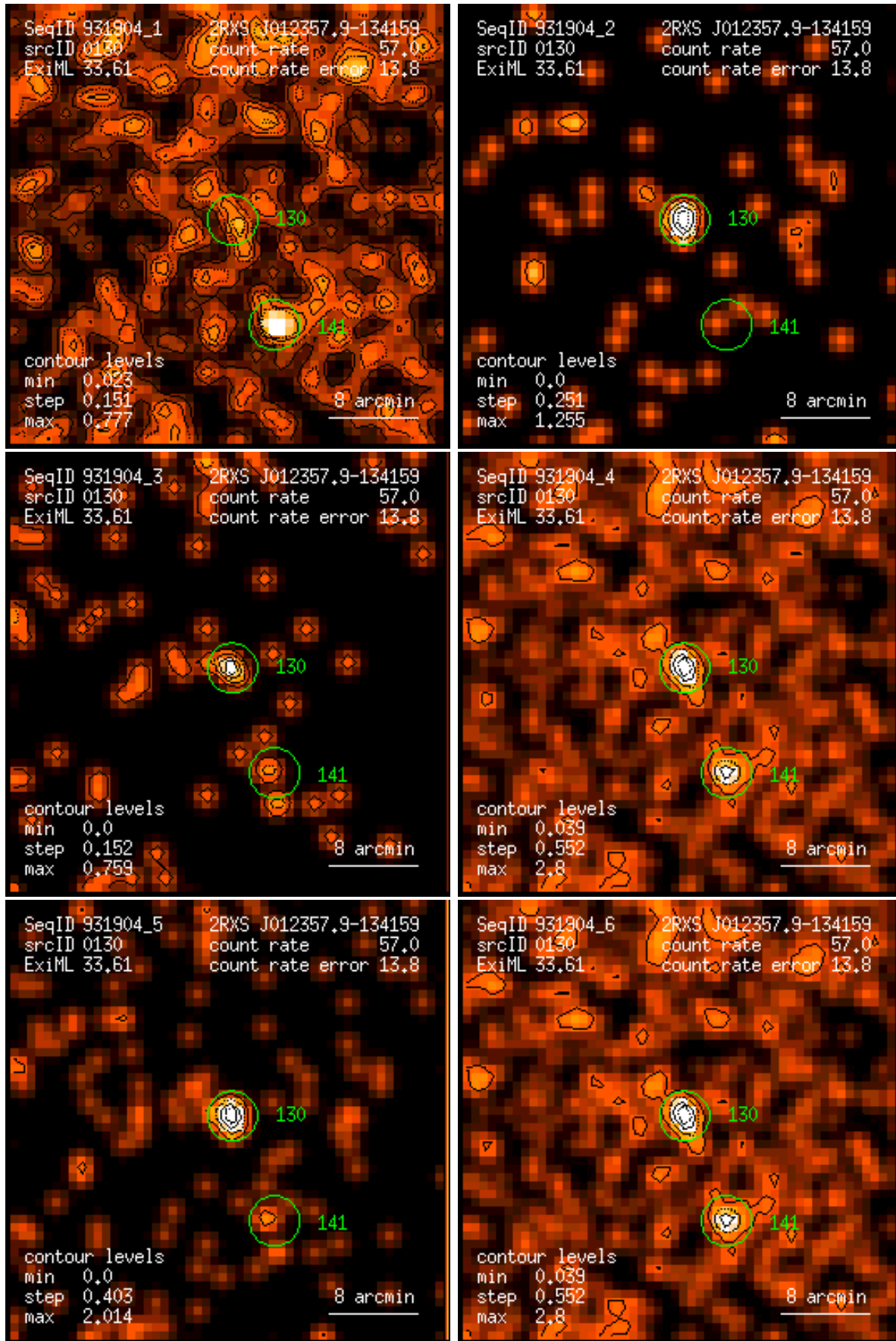
Figure 130: RASS 931904: detection 0130: band rate images, Gaussian filter: (1) PSPC channels 11 – 41, (2) 52 – 90, (3) 91 – 201, (4) 11 – 235, (5) 52 – 201, (6) 11 – 201. Broad band rates in counts/ks. Band rate contour levels in counts/ks/arcmin 2 .
