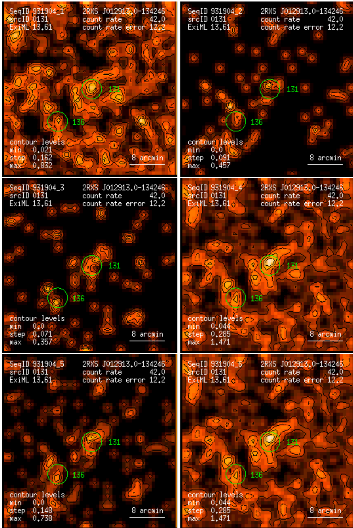
Figure 131: RASS 931904: detection 0131: band rate images, Gaussian filter: (1) PSPC channels 11 – 41, (2) 52 – 90, (3) 91 – 201, (4) 11 – 235, (5) 52 – 201, (6) 11 – 201. Broad band rates in counts/ks. Band rate contour levels in counts/ks/arcmin 2 .
