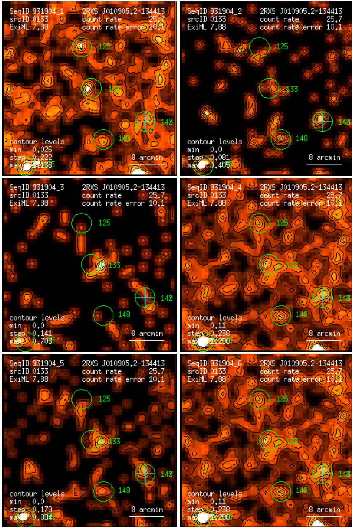
Figure 133: RASS 931904: detection 0133: band rate images, Gaussian filter: (1) PSPC channels 11 – 41, (2) 52 – 90, (3) 91 – 201, (4) 11 – 235, (5) 52 – 201, (6) 11 – 201. Broad band rates in counts/ks. Band rate contour levels in counts/ks/arcmin 2 .
