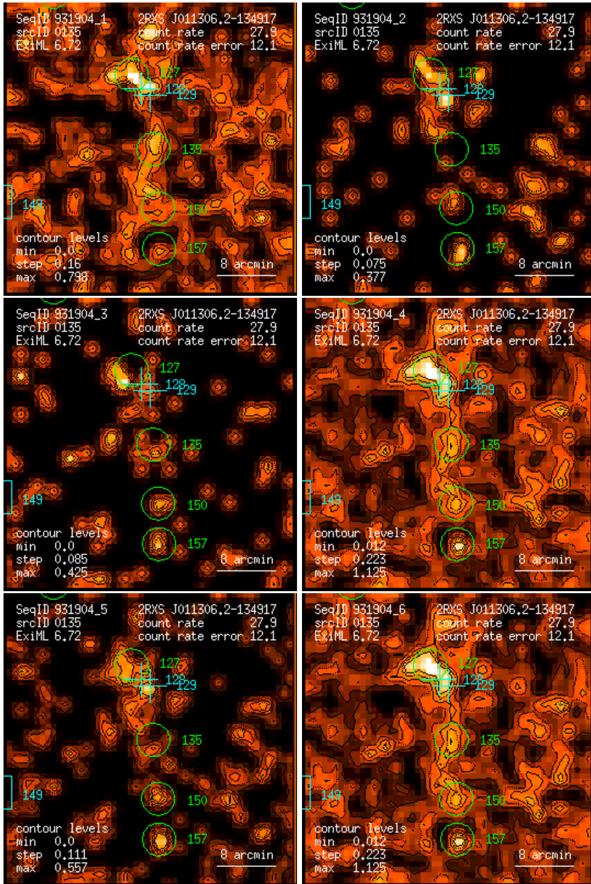
Figure 135: RASS 931904: detection 0135: band rate images, Gaussian filter: (1) PSPC channels 11 – 41, (2) 52 – 90, (3) 91 – 201, (4) 11 – 235, (5) 52 – 201, (6) 11 – 201. Broad band rates in counts/ks. Band rate contour levels in counts/ks/arcmin 2 .
