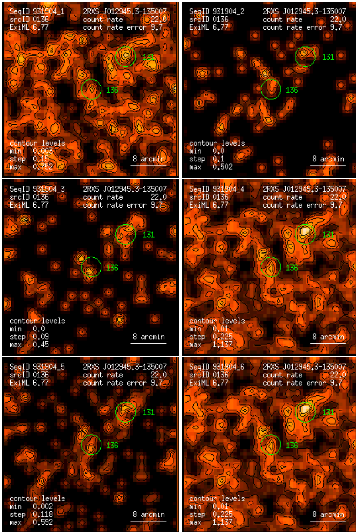
Figure 136: RASS 931904: detection 0136: band rate images, Gaussian filter: (1) PSPC channels 11 – 41, (2) 52 – 90, (3) 91 – 201, (4) 11 – 235, (5) 52 – 201, (6) 11 – 201. Broad band rates in counts/ks. Band rate contour levels in counts/ks/arcmin 2 .
