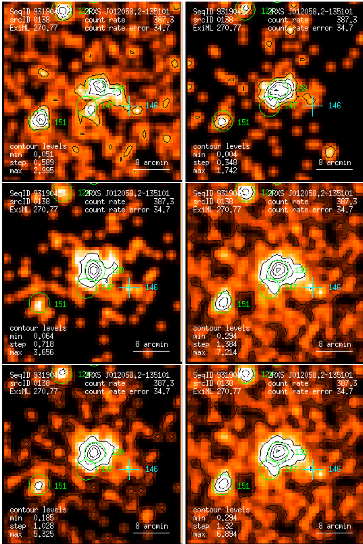
Figure 138: RASS 931904: detection 0138: band rate images, Gaussian filter: (1) PSPC channels 11 – 41, (2) 52 – 90, (3) 91 – 201, (4) 11 – 235, (5) 52 – 201, (6) 11 – 201. Broad band rates in counts/ks. Band rate contour levels in counts/ks/arcmin 2 .
