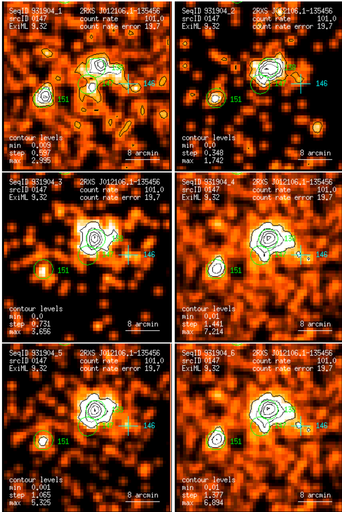
Figure 147: RASS 931904: detection 0147: band rate images, Gaussian filter: (1) PSPC channels 11 – 41, (2) 52 – 90, (3) 91 – 201, (4) 11 – 235, (5) 52 – 201, (6) 11 – 201. Broad band rates in counts/ks. Band rate contour levels in counts/ks/arcmin 2 .
