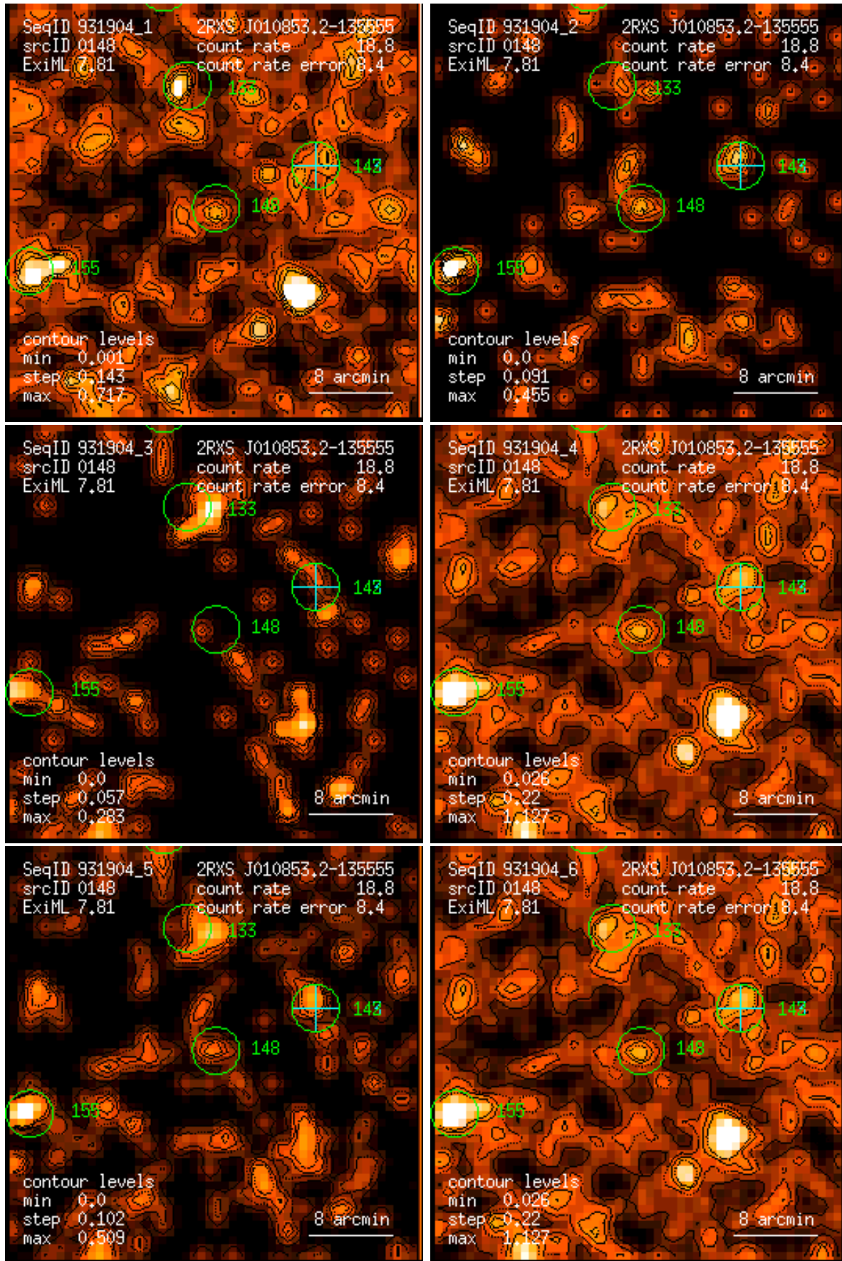
Figure 148: RASS 931904: detection 0148: band rate images, Gaussian filter: (1) PSPC channels 11 – 41, (2) 52 – 90, (3) 91 – 201, (4) 11 – 235, (5) 52 – 201, (6) 11 – 201. Broad band rates in counts/ks. Band rate contour levels in counts/ks/arcmin 2 .
