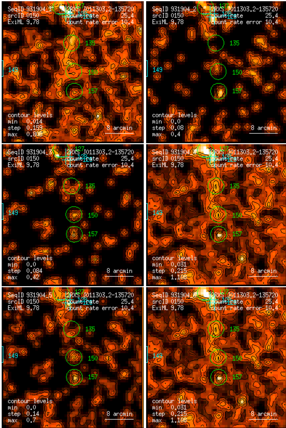
Figure 150: RASS 931904: detection 0150: band rate images, Gaussian filter: (1) PSPC channels 11 – 41, (2) 52 – 90, (3) 91 – 201, (4) 11 – 235, (5) 52 – 201, (6) 11 – 201. Broad band rates in counts/ks. Band rate contour levels in counts/ks/arcmin 2 .
