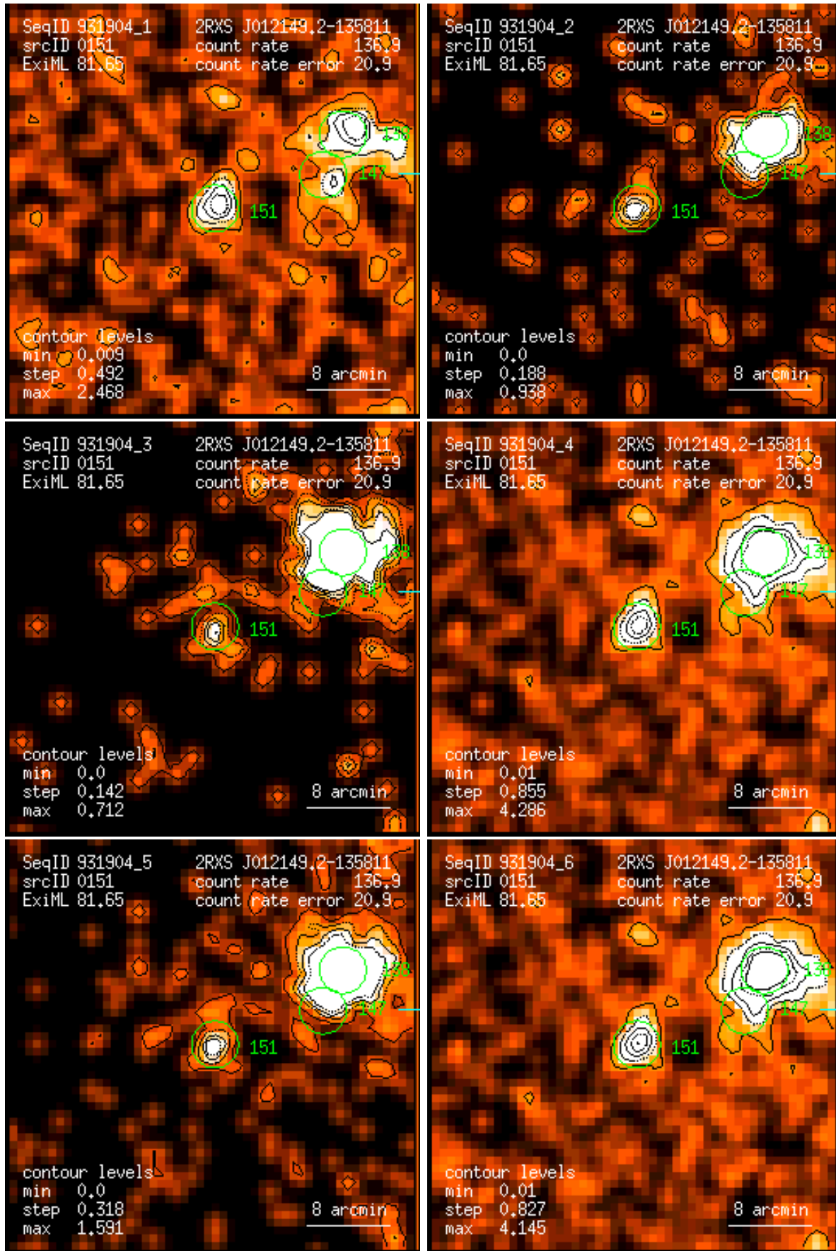
Figure 151: RASS 931904: detection 0151: band rate images, Gaussian filter: (1) PSPC channels 11 – 41, (2) 52 – 90, (3) 91 – 201, (4) 11 – 235, (5) 52 – 201, (6) 11 – 201. Broad band rates in counts/ks. Band rate contour levels in counts/ks/arcmin 2 .
