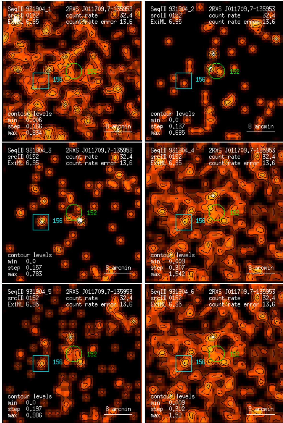
Figure 152: RASS 931904: detection 0152: band rate images, Gaussian filter: (1) PSPC channels 11 – 41, (2) 52 – 90, (3) 91 – 201, (4) 11 – 235, (5) 52 – 201, (6) 11 – 201. Broad band rates in counts/ks. Band rate contour levels in counts/ks/arcmin 2 .
