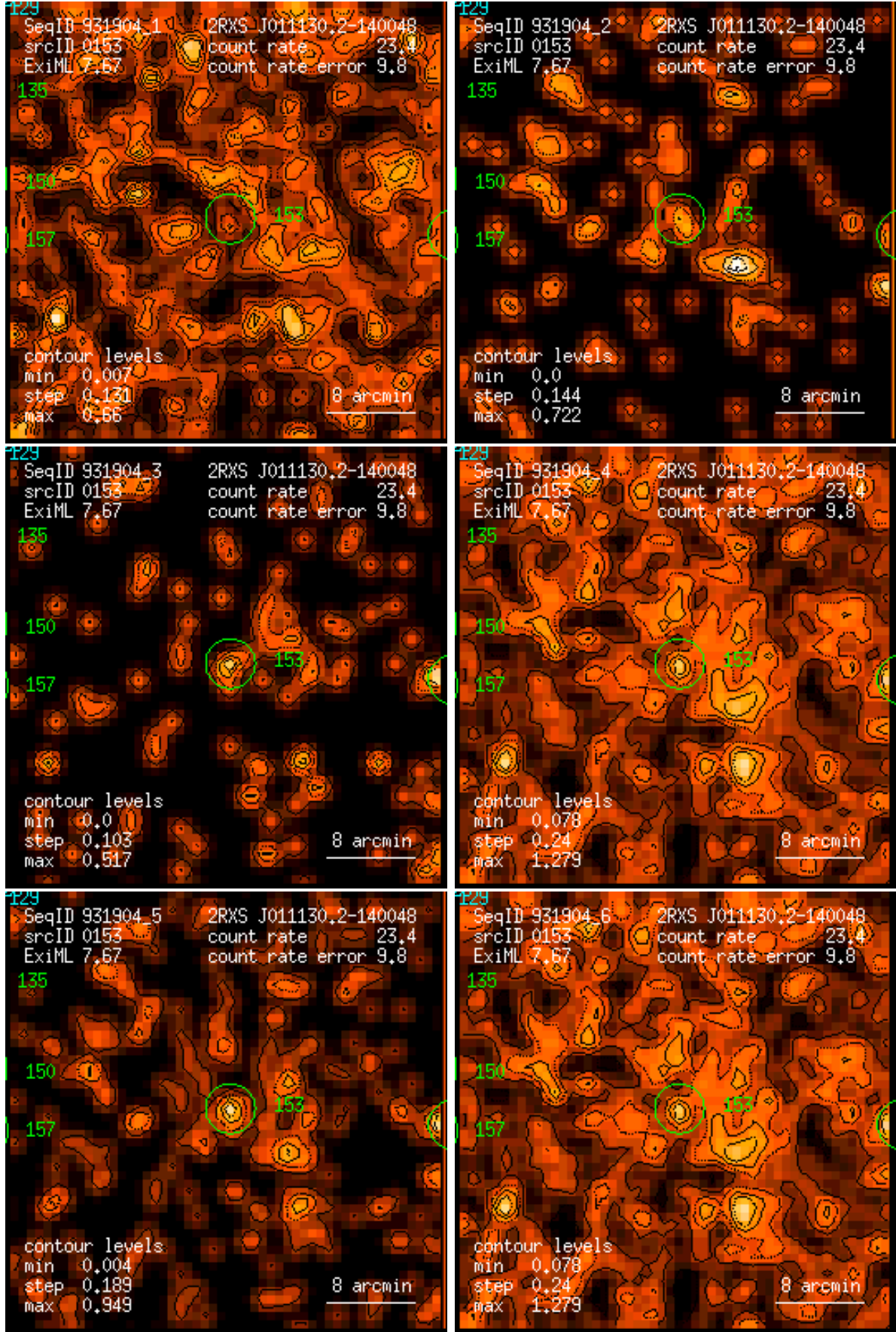
Figure 153: RASS 931904: detection 0153: band rate images, Gaussian filter: (1) PSPC channels 11 – 41, (2) 52 – 90, (3) 91 – 201, (4) 11 – 235, (5) 52 – 201, (6) 11 – 201. Broad band rates in counts/ks. Band rate contour levels in counts/ks/arcmin 2 .
