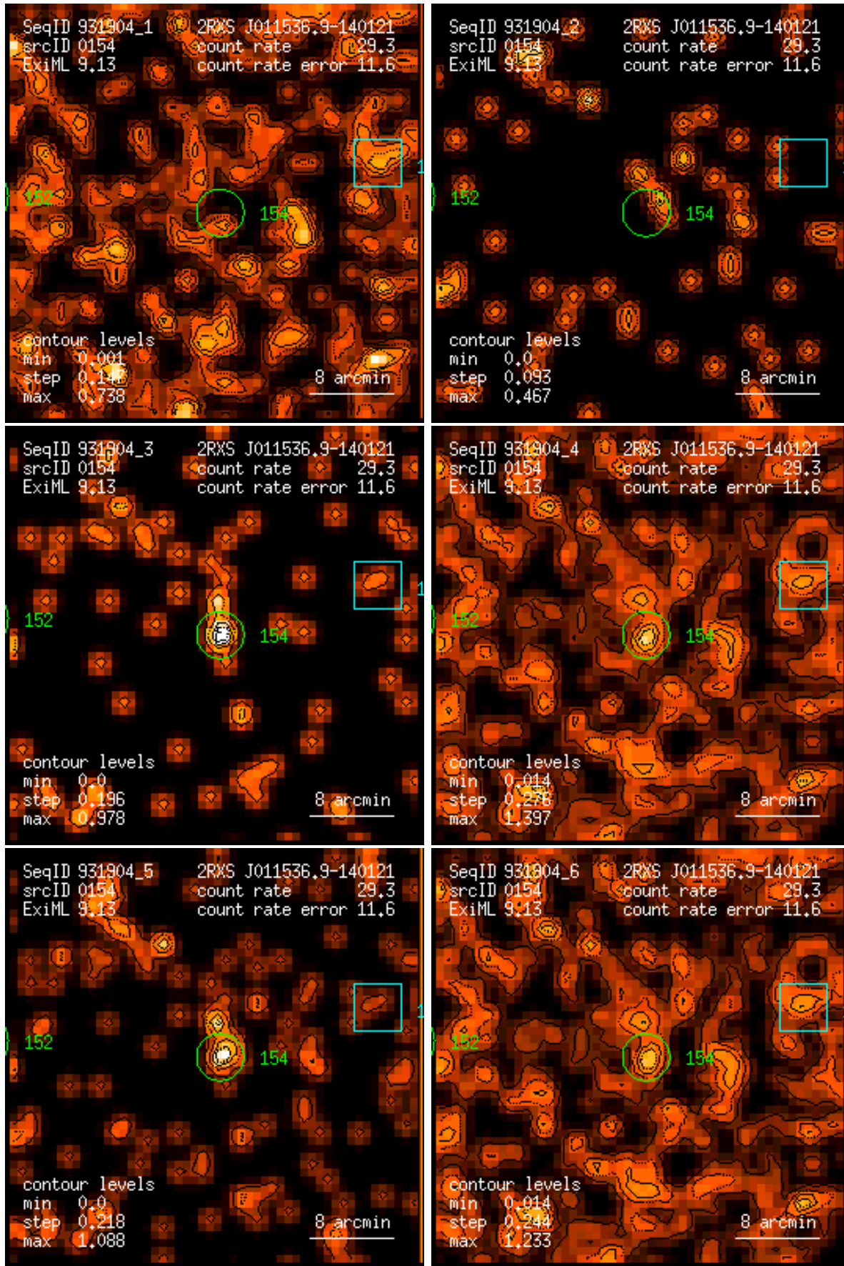
Figure 154: RASS 931904: detection 0154: band rate images, Gaussian filter: (1) PSPC channels 11 – 41, (2) 52 – 90, (3) 91 – 201, (4) 11 – 235, (5) 52 – 201, (6) 11 – 201. Broad band rates in counts/ks. Band rate contour levels in counts/ks/arcmin 2 .
