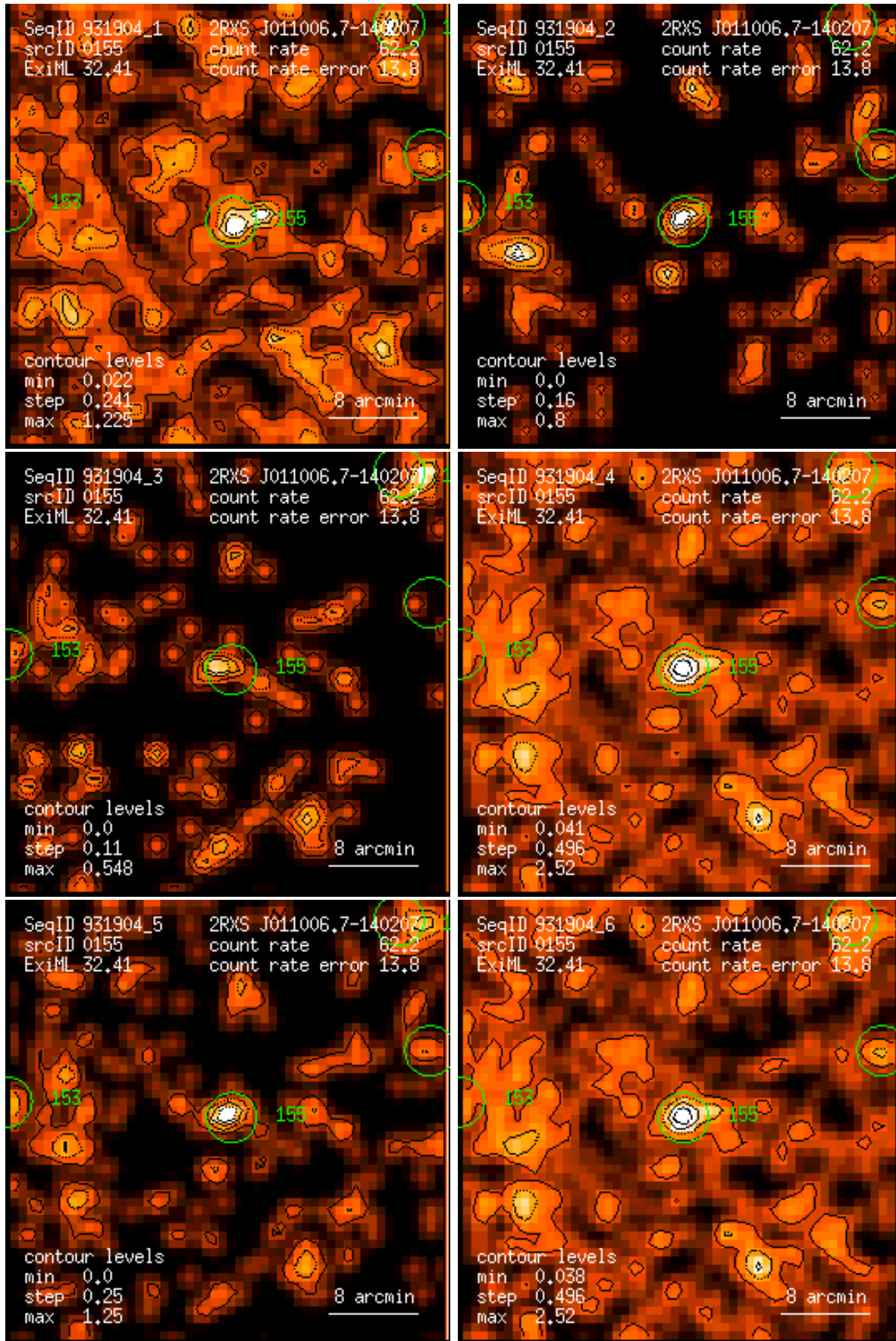
Figure 155: RASS 931904: detection 0155: band rate images, Gaussian filter: (1) PSPC channels 11 – 41, (2) 52 – 90, (3) 91 – 201, (4) 11 – 235, (5) 52 – 201, (6) 11 – 201. Broad band rates in counts/ks. Band rate contour levels in counts/ks/arcmin 2 .
