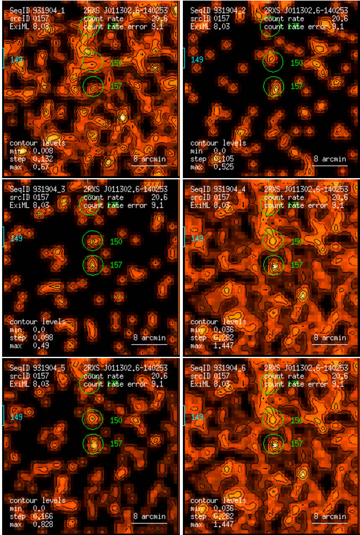
Figure 157: RASS 931904: detection 0157: band rate images, Gaussian filter: (1) PSPC channels 11 – 41, (2) 52 – 90, (3) 91 – 201, (4) 11 – 235, (5) 52 – 201, (6) 11 – 201. Broad band rates in counts/ks. Band rate contour levels in counts/ks/arcmin 2 .
