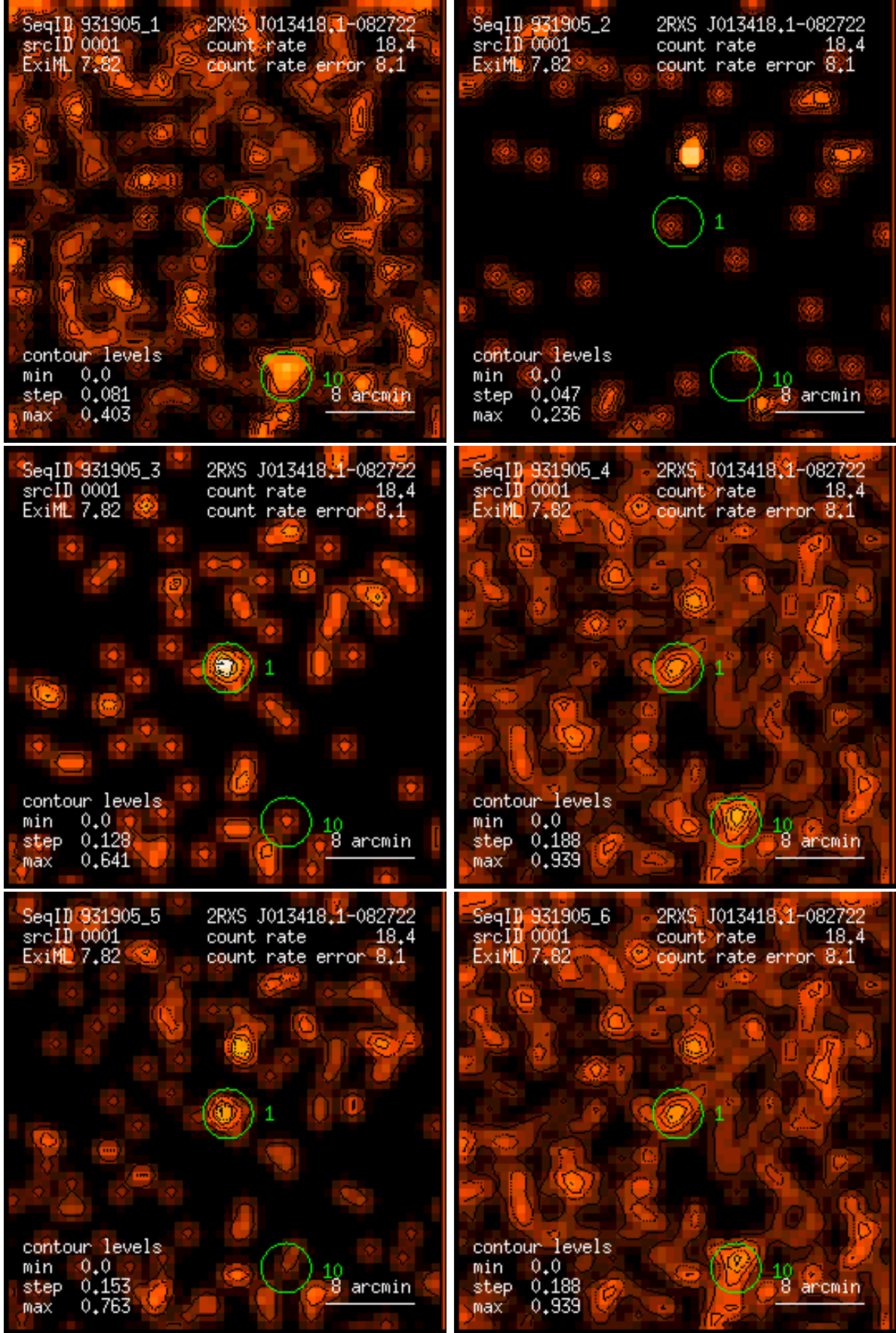
Figure 1: RASS 931905: detection 0001: band rate images, Gaussian filter: (1) PSPC channels 11 – 41, (2) 52 – 90, (3) 91 – 201, (4) 11 – 235, (5) 52 – 201, (6) 11 – 201. Broad band rates in counts/ks. Band rate contour levels in counts/ks/arcmin 2 .
