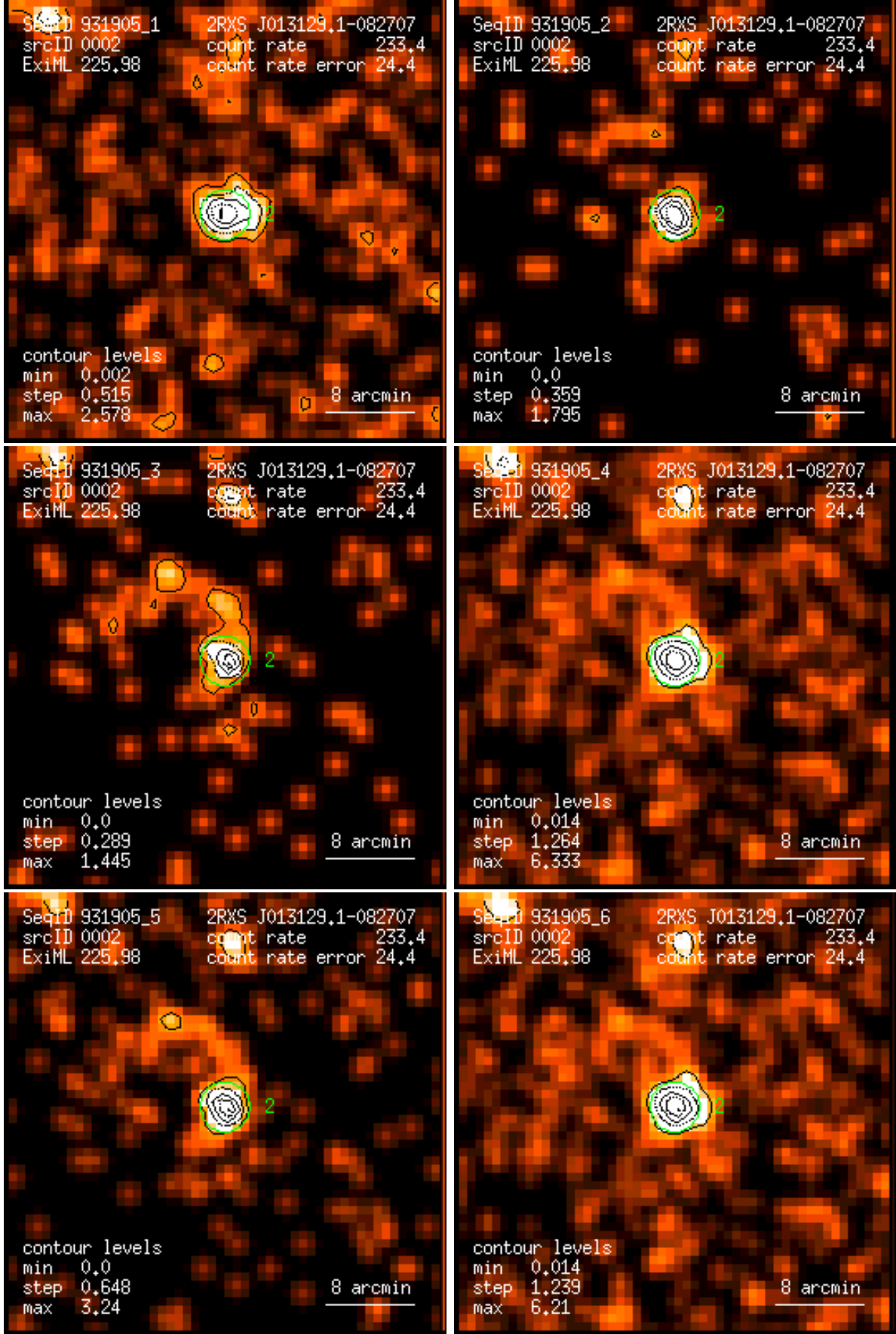
Figure 2: RASS 931905: detection 0002: band rate images, Gaussian filter: (1) PSPC channels 11 – 41, (2) 52 – 90, (3) 91 – 201, (4) 11 – 235, (5) 52 – 201, (6) 11 – 201. Broad band rates in counts/ks. Band rate contour levels in counts/ks/arcmin 2 .
