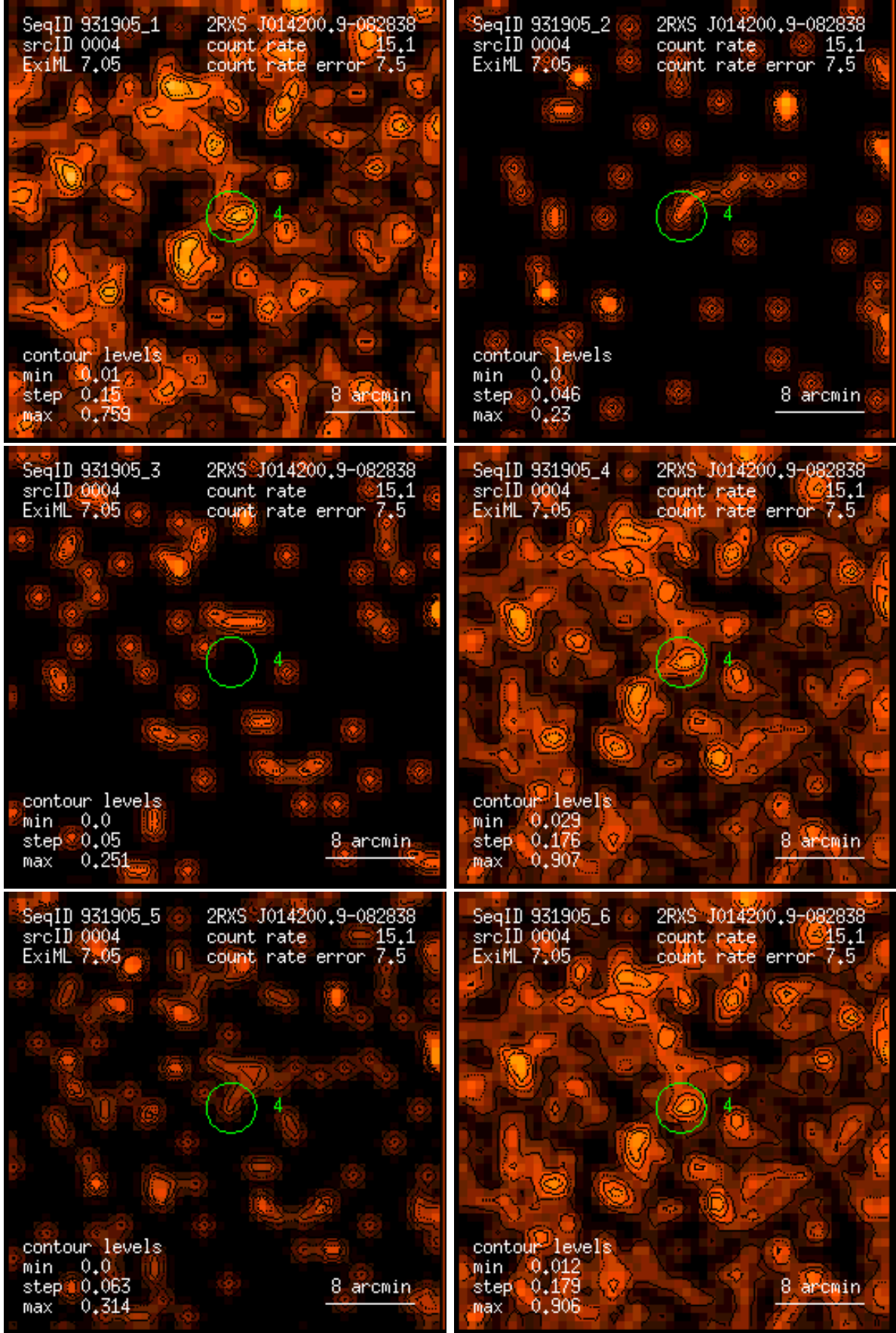
Figure 4: RASS 931905: detection 0004: band rate images, Gaussian filter: (1) PSPC channels 11 – 41, (2) 52 – 90, (3) 91 – 201, (4) 11 – 235, (5) 52 – 201, (6) 11 – 201. Broad band rates in counts/ks. Band rate contour levels in counts/ks/arcmin 2 .
