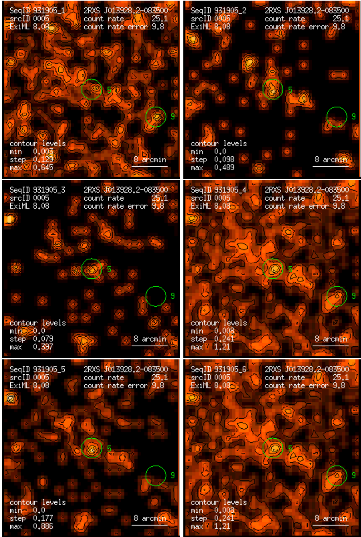
Figure 5: RASS 931905: detection 0005: band rate images, Gaussian filter: (1) PSPC channels 11 – 41, (2) 52 – 90, (3) 91 – 201, (4) 11 – 235, (5) 52 – 201, (6) 11 – 201. Broad band rates in counts/ks. Band rate contour levels in counts/ks/arcmin 2 .
