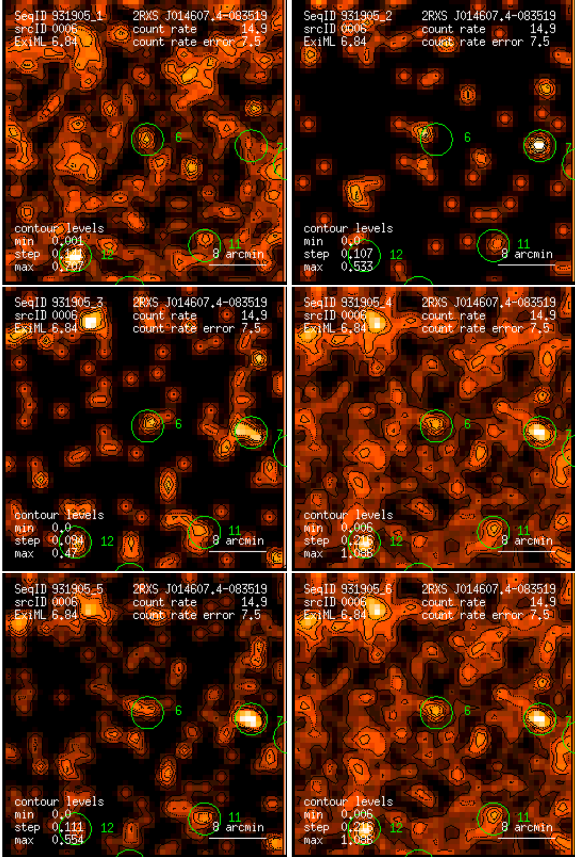
Figure 6: RASS 931905: detection 0006: band rate images, Gaussian filter: (1) PSPC channels 11 – 41, (2) 52 – 90, (3) 91 – 201, (4) 11 – 235, (5) 52 – 201, (6) 11 – 201. Broad band rates in counts/ks. Band rate contour levels in counts/ks/arcmin 2 .
