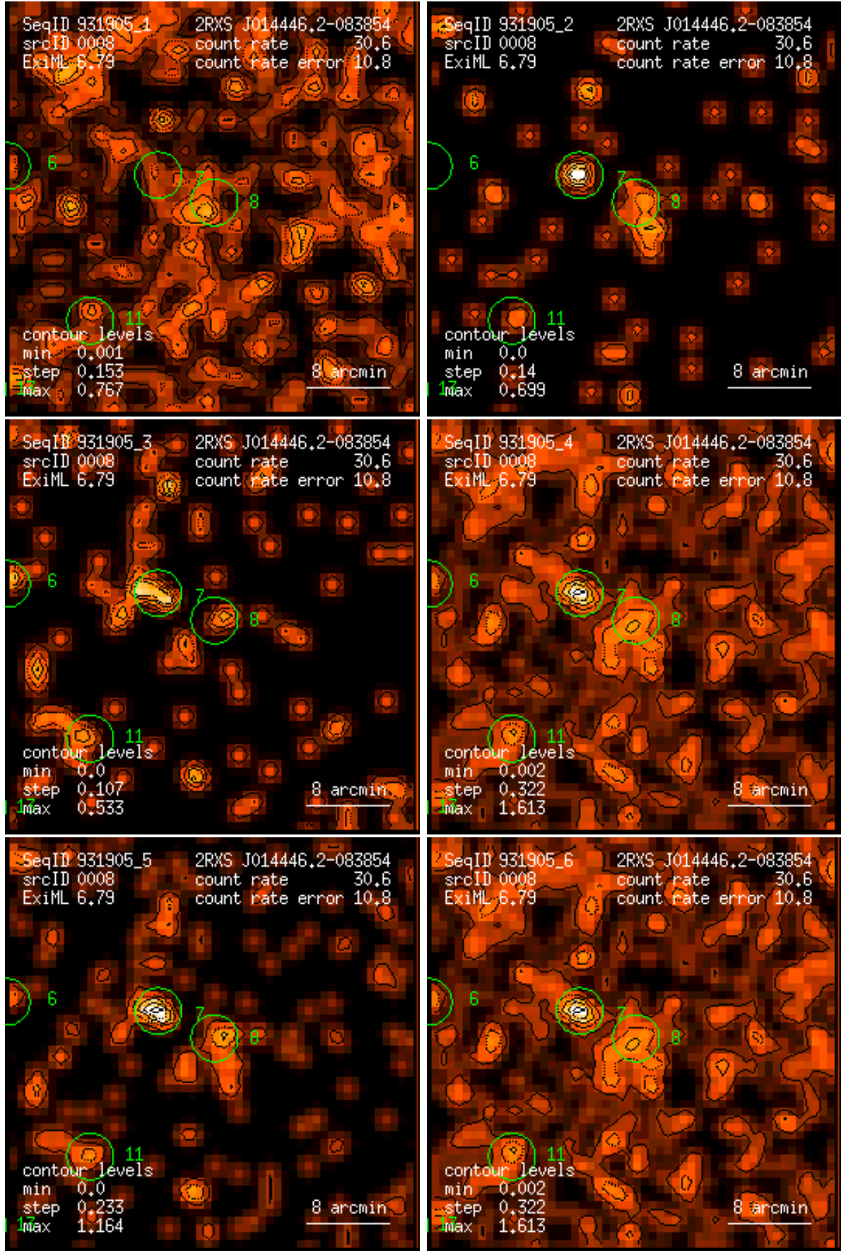
Figure 8: RASS 931905: detection 0008: band rate images, Gaussian filter: (1) PSPC channels 11 – 41, (2) 52 – 90, (3) 91 – 201, (4) 11 – 235, (5) 52 – 201, (6) 11 – 201. Broad band rates in counts/ks. Band rate contour levels in counts/ks/arcmin 2 .
