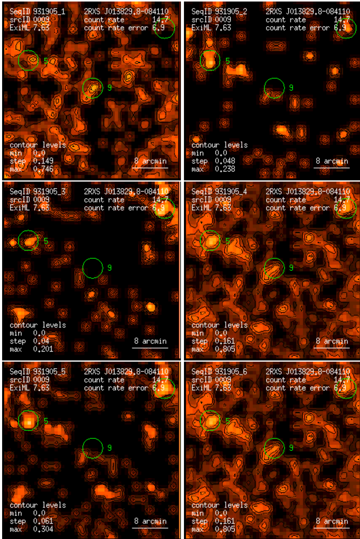
Figure 9: RASS 931905: detection 0009: band rate images, Gaussian filter: (1) PSPC channels 11 – 41, (2) 52 – 90, (3) 91 – 201, (4) 11 – 235, (5) 52 – 201, (6) 11 – 201. Broad band rates in counts/ks. Band rate contour levels in counts/ks/arcmin 2 .
