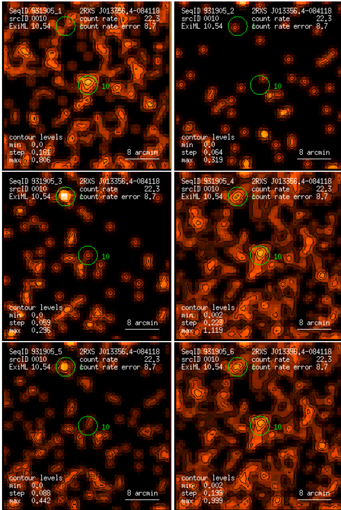
Figure 10: RASS 931905: detection 0010: band rate images, Gaussian filter: (1) PSPC channels 11 – 41, (2) 52 – 90, (3) 91 – 201, (4) 11 – 235, (5) 52 – 201, (6) 11 – 201. Broad band rates in counts/ks. Band rate contour levels in counts/ks/arcmin 2 .
