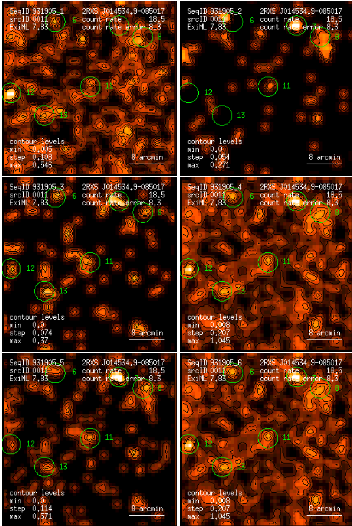
Figure 11: RASS 931905: detection 0011: band rate images, Gaussian filter: (1) PSPC channels 11 – 41, (2) 52 – 90, (3) 91 – 201, (4) 11 – 235, (5) 52 – 201, (6) 11 – 201. Broad band rates in counts/ks. Band rate contour levels in counts/ks/arcmin 2 .
