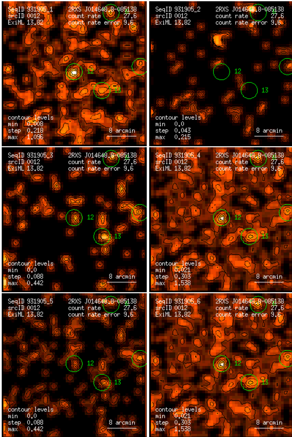
Figure 12: RASS 931905: detection 0012: band rate images, Gaussian filter: (1) PSPC channels 11 – 41, (2) 52 – 90, (3) 91 – 201, (4) 11 – 235, (5) 52 – 201, (6) 11 – 201. Broad band rates in counts/ks. Band rate contour levels in counts/ks/arcmin 2 .
