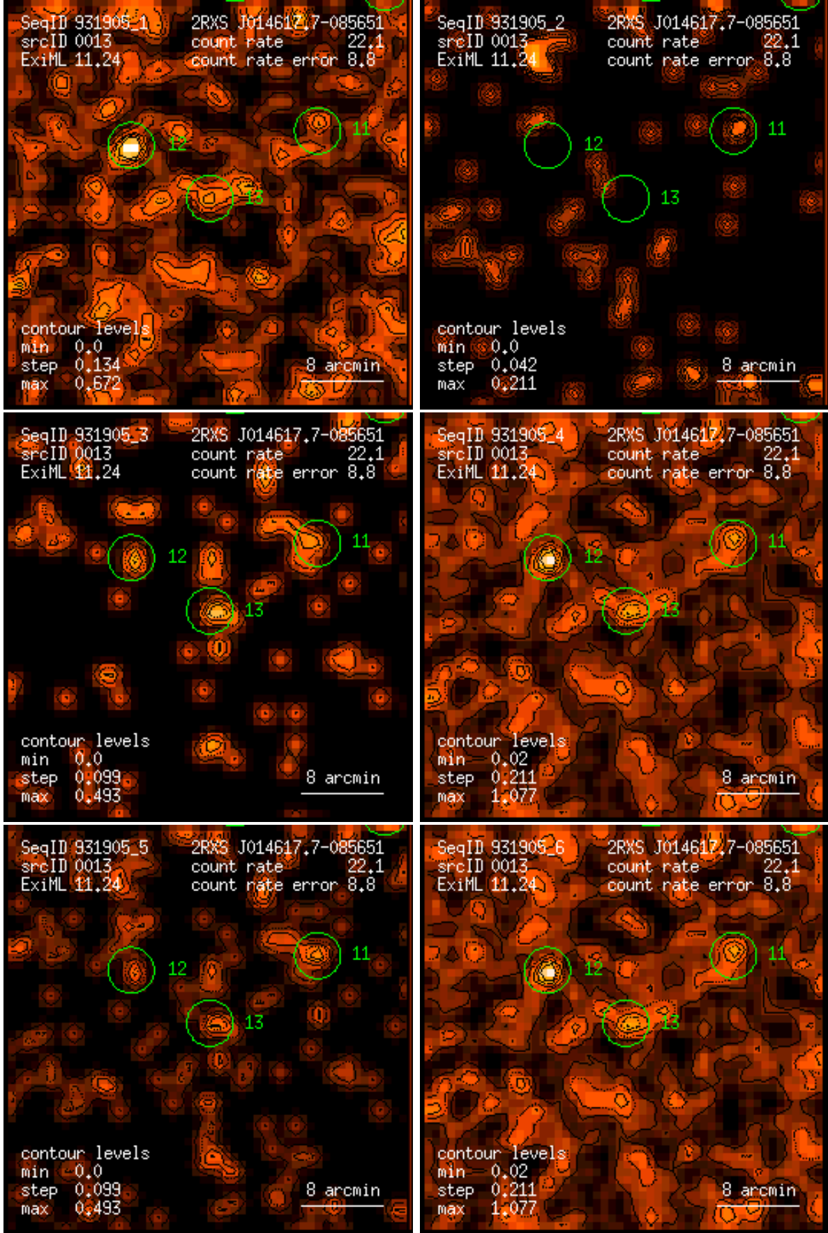
Figure 13: RASS 931905: detection 0013: band rate images, Gaussian filter: (1) PSPC channels 11 – 41, (2) 52 – 90, (3) 91 – 201, (4) 11 – 235, (5) 52 – 201, (6) 11 – 201. Broad band rates in counts/ks. Band rate contour levels in counts/ks/arcmin 2 .
