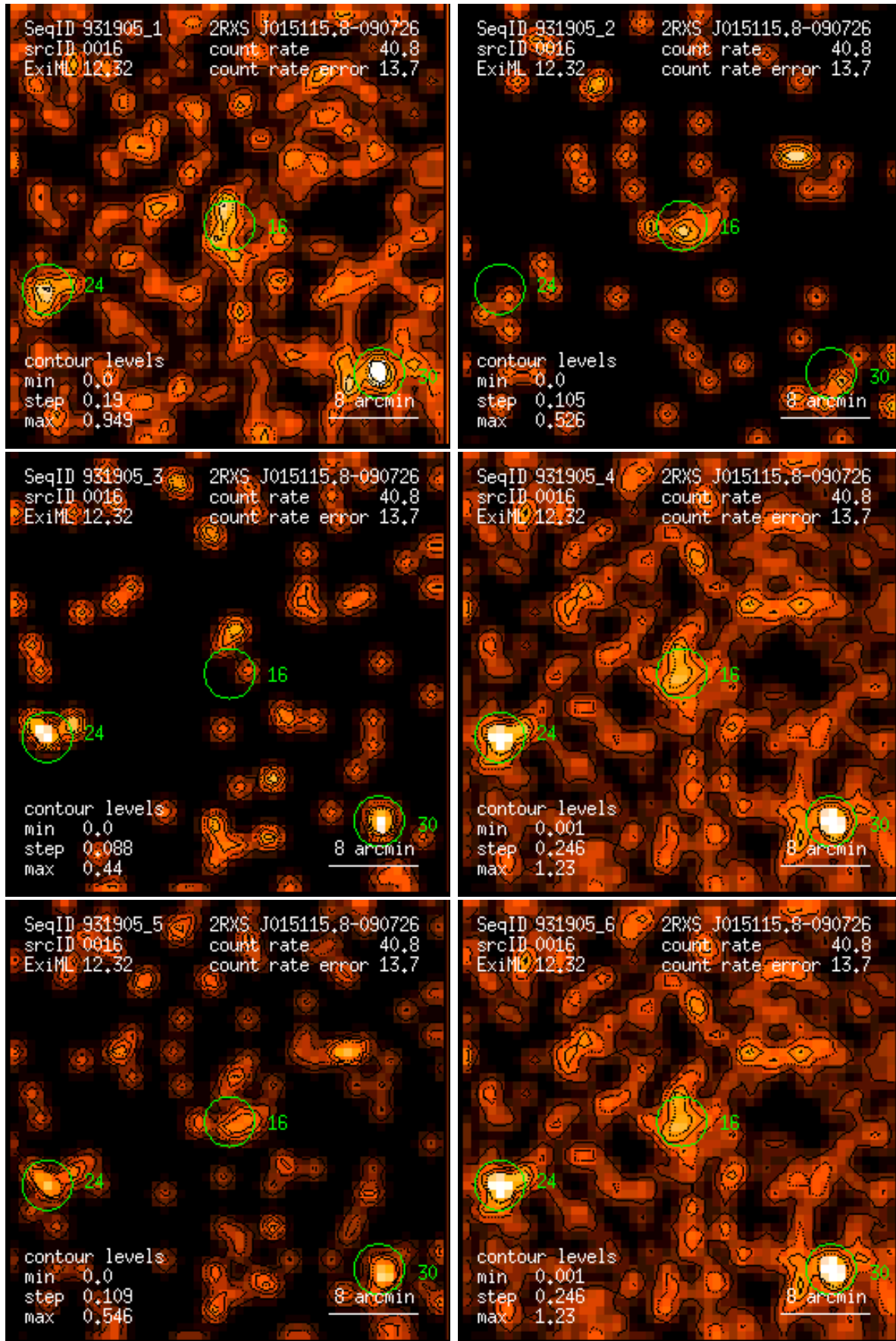
Figure 16: RASS 931905: detection 0016: band rate images, Gaussian filter: (1) PSPC channels 11 – 41, (2) 52 – 90, (3) 91 – 201, (4) 11 – 235, (5) 52 – 201, (6) 11 – 201. Broad band rates in counts/ks. Band rate contour levels in counts/ks/arcmin 2 .
