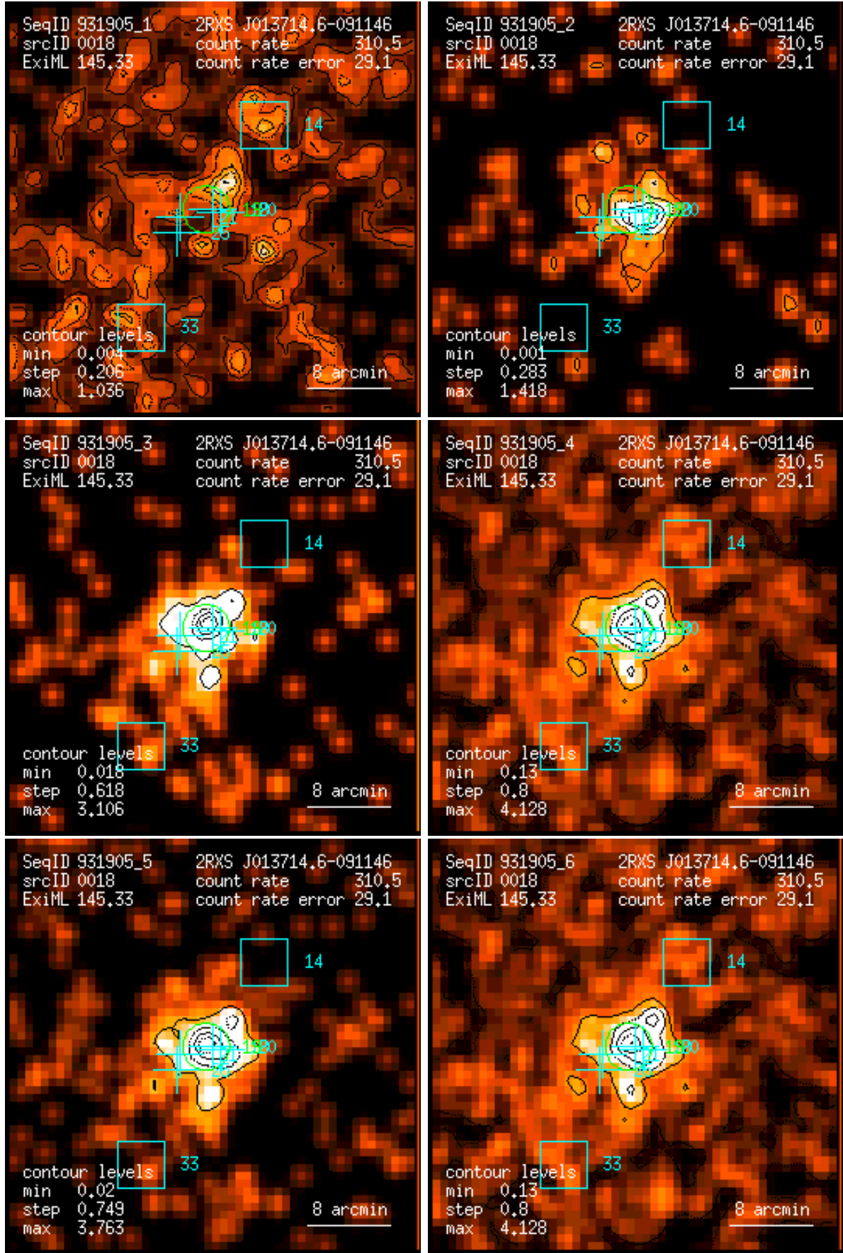
Figure 18: RASS 931905: detection 0018: band rate images, Gaussian filter: (1) PSPC channels 11 – 41, (2) 52 – 90, (3) 91 – 201, (4) 11 – 235, (5) 52 – 201, (6) 11 – 201. Broad band rates in counts/ks. Band rate contour levels in counts/ks/arcmin 2 .
