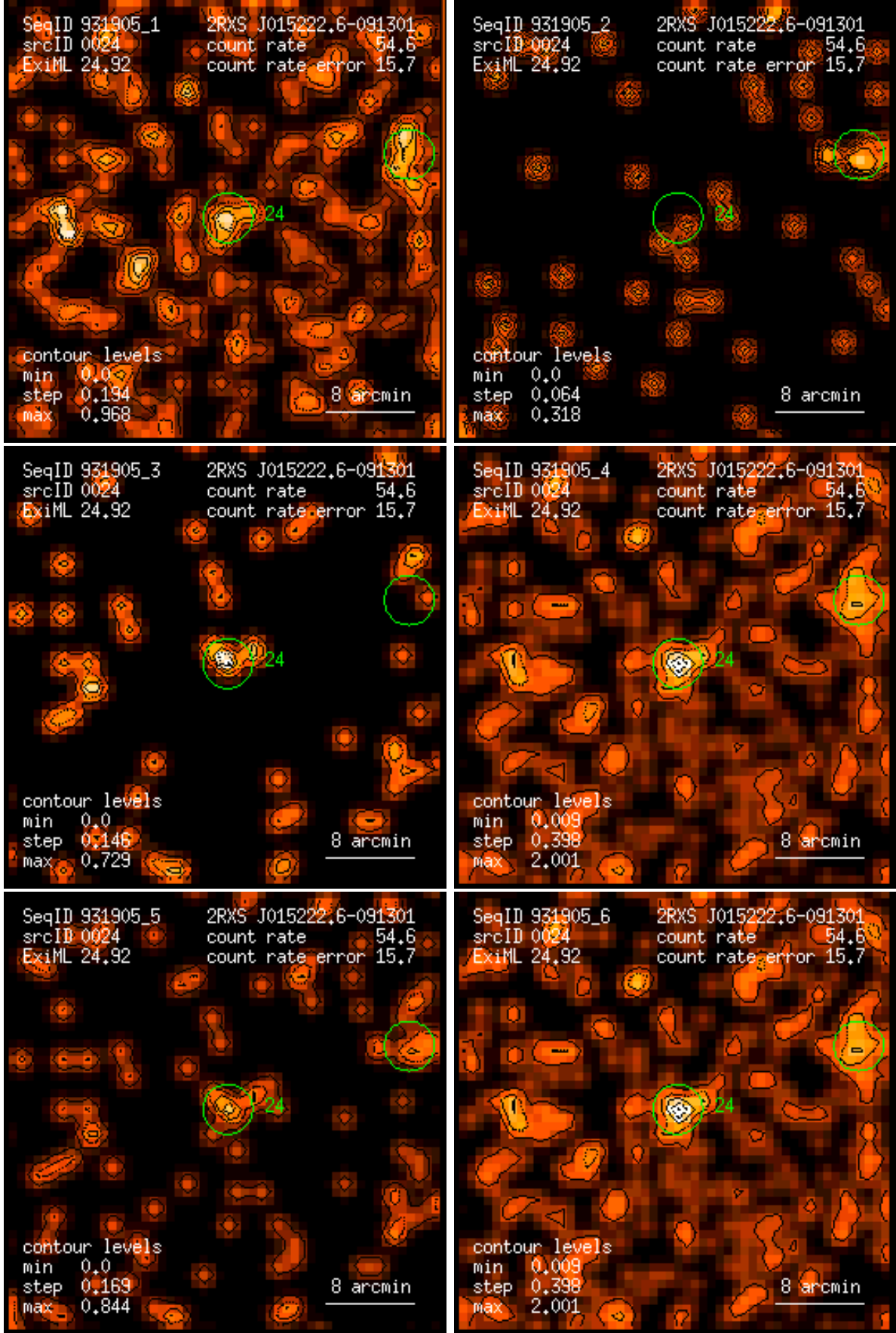
Figure 24: RASS 931905: detection 0024: band rate images, Gaussian filter: (1) PSPC channels 11 – 41, (2) 52 – 90, (3) 91 – 201, (4) 11 – 235, (5) 52 – 201, (6) 11 – 201. Broad band rates in counts/ks. Band rate contour levels in counts/ks/arcmin 2 .
