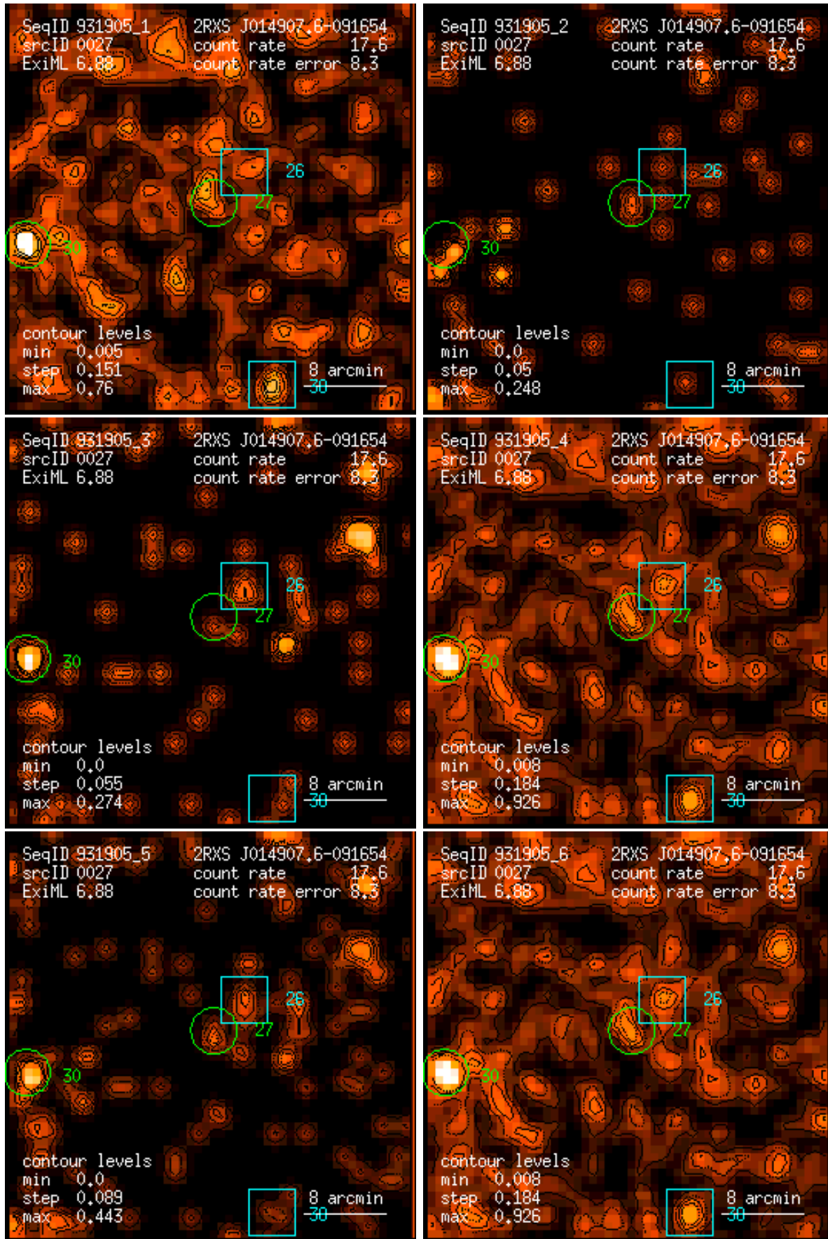
Figure 27: RASS 931905: detection 0027: band rate images, Gaussian filter: (1) PSPC channels 11 – 41, (2) 52 – 90, (3) 91 – 201, (4) 11 – 235, (5) 52 – 201, (6) 11 – 201. Broad band rates in counts/ks. Band rate contour levels in counts/ks/arcmin 2 .
