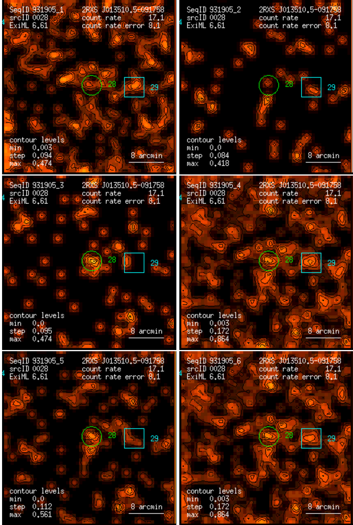
Figure 28: RASS 931905: detection 0028: band rate images, Gaussian filter: (1) PSPC channels 11 – 41, (2) 52 – 90, (3) 91 – 201, (4) 11 – 235, (5) 52 – 201, (6) 11 – 201. Broad band rates in counts/ks. Band rate contour levels in counts/ks/arcmin 2 .
