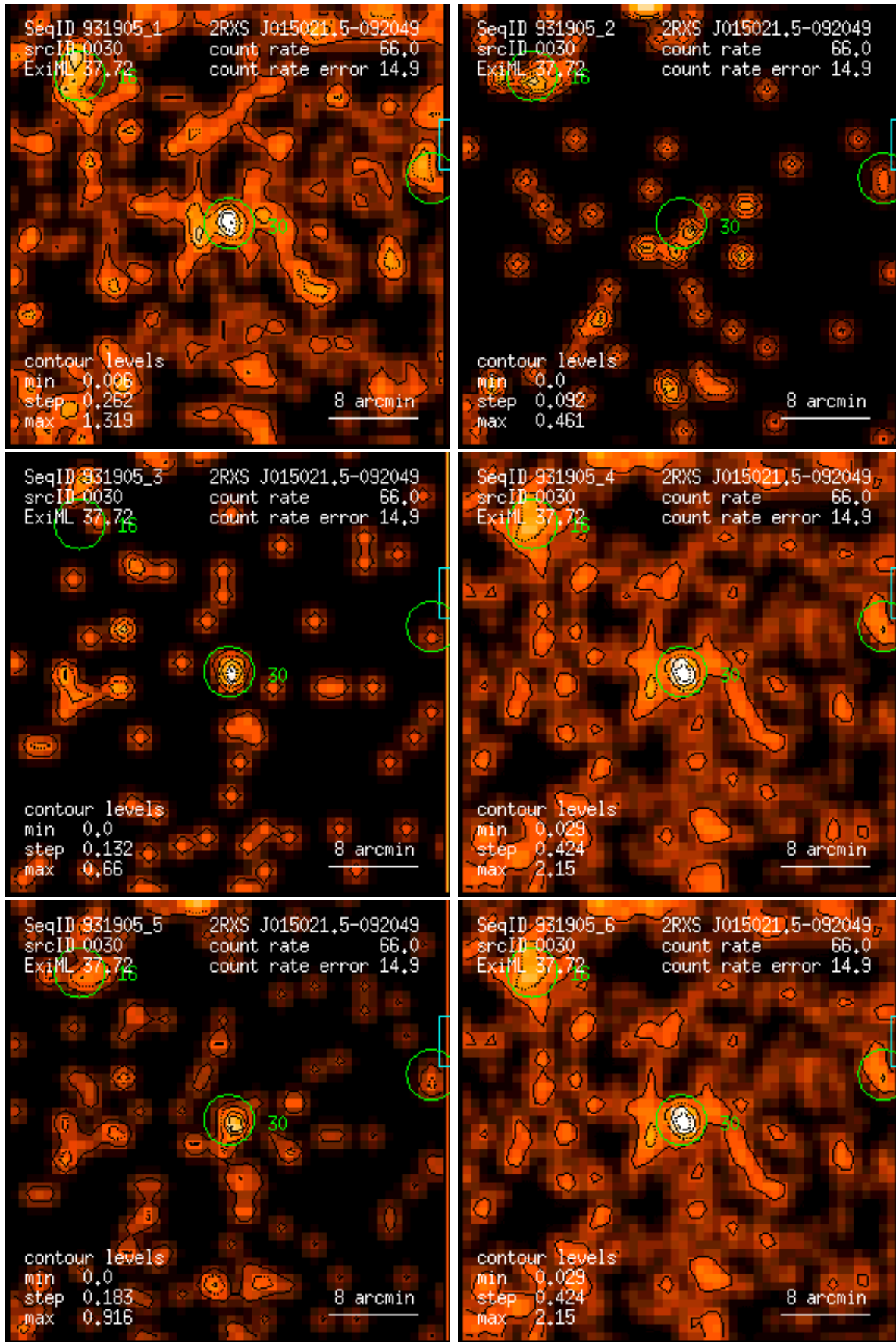
Figure 30: RASS 931905: detection 0030: band rate images, Gaussian filter: (1) PSPC channels 11 – 41, (2) 52 – 90, (3) 91 – 201, (4) 11 – 235, (5) 52 – 201, (6) 11 – 201. Broad band rates in counts/ks. Band rate contour levels in counts/ks/arcmin 2 .
