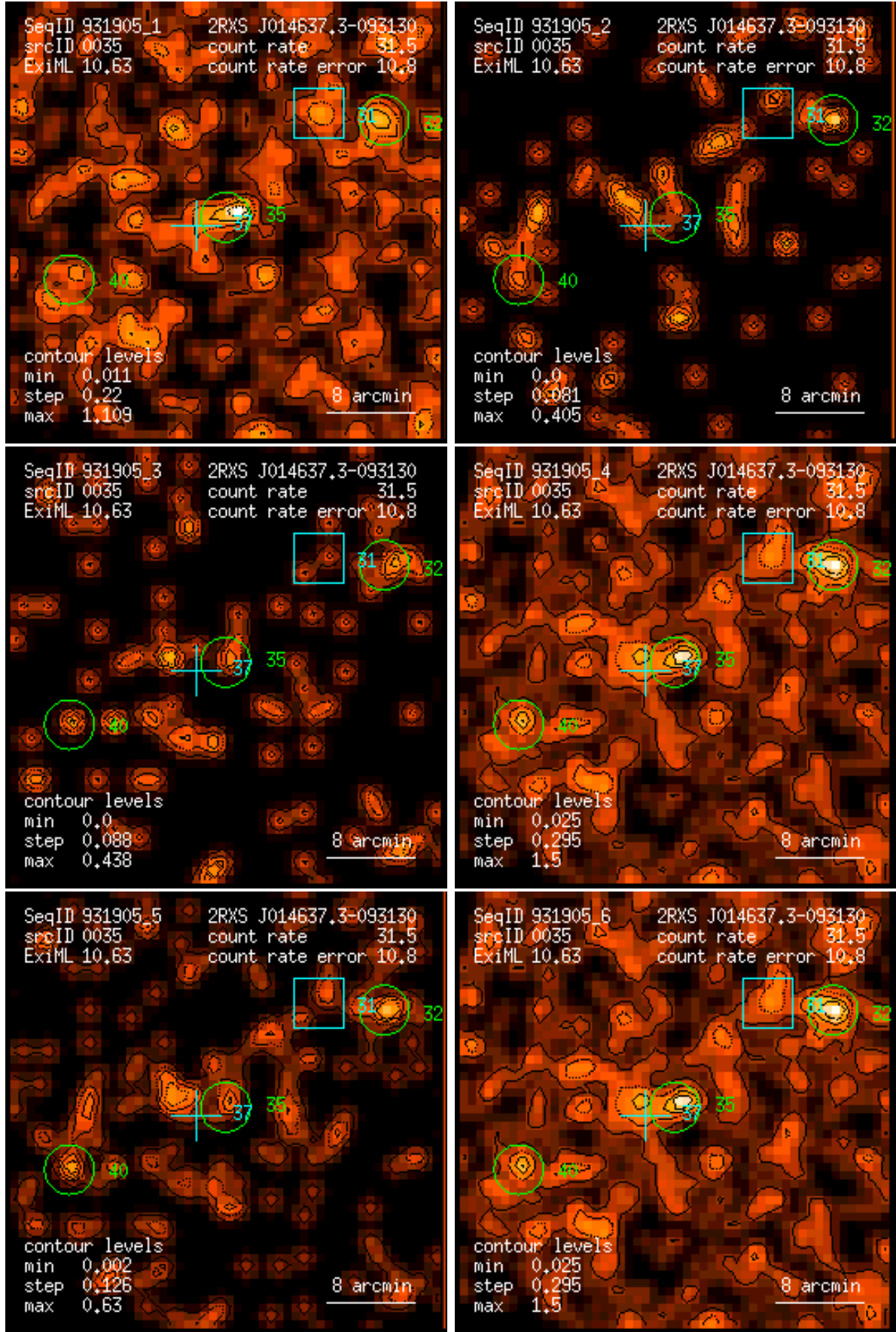
Figure 35: RASS 931905: detection 0035: band rate images, Gaussian filter: (1) PSPC channels 11 – 41, (2) 52 – 90, (3) 91 – 201, (4) 11 – 235, (5) 52 – 201, (6) 11 – 201. Broad band rates in counts/ks. Band rate contour levels in counts/ks/arcmin 2 .
