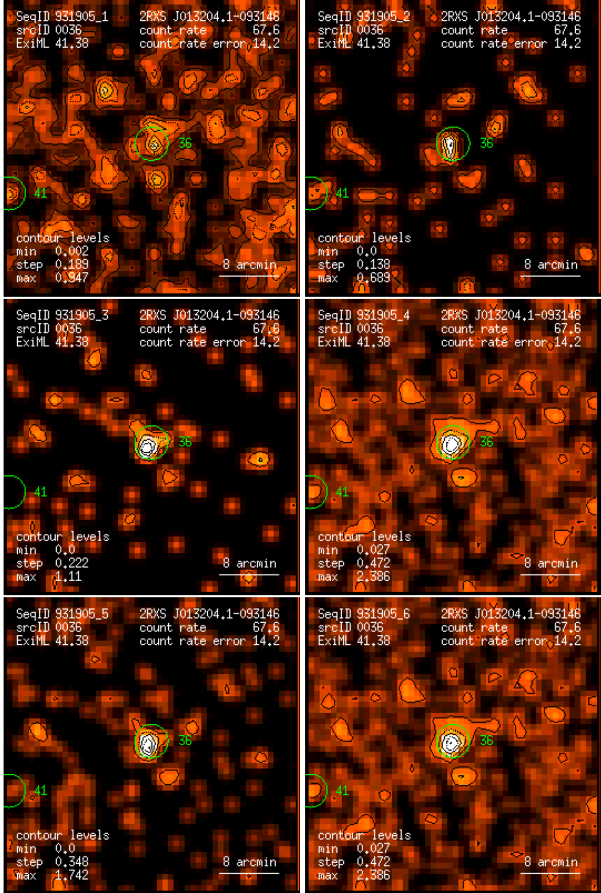
Figure 36: RASS 931905: detection 0036: band rate images, Gaussian filter: (1) PSPC channels 11 – 41, (2) 52 – 90, (3) 91 – 201, (4) 11 – 235, (5) 52 – 201, (6) 11 – 201. Broad band rates in counts/ks. Band rate contour levels in counts/ks/arcmin 2 .
