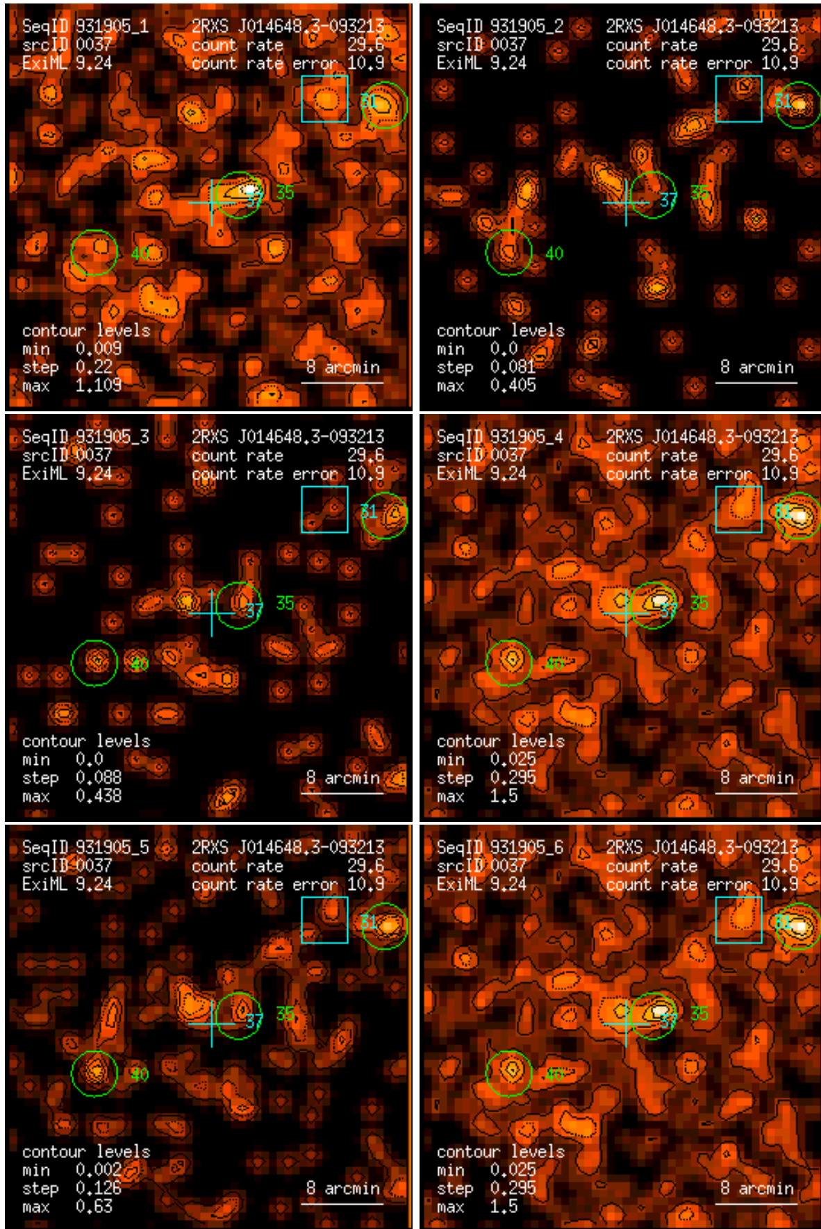
Figure 37: RASS 931905: detection 0037: band rate images, Gaussian filter: (1) PSPC channels 11 – 41, (2) 52 – 90, (3) 91 – 201, (4) 11 – 235, (5) 52 – 201, (6) 11 – 201. Broad band rates in counts/ks. Band rate contour levels in counts/ks/arcmin 2 .
