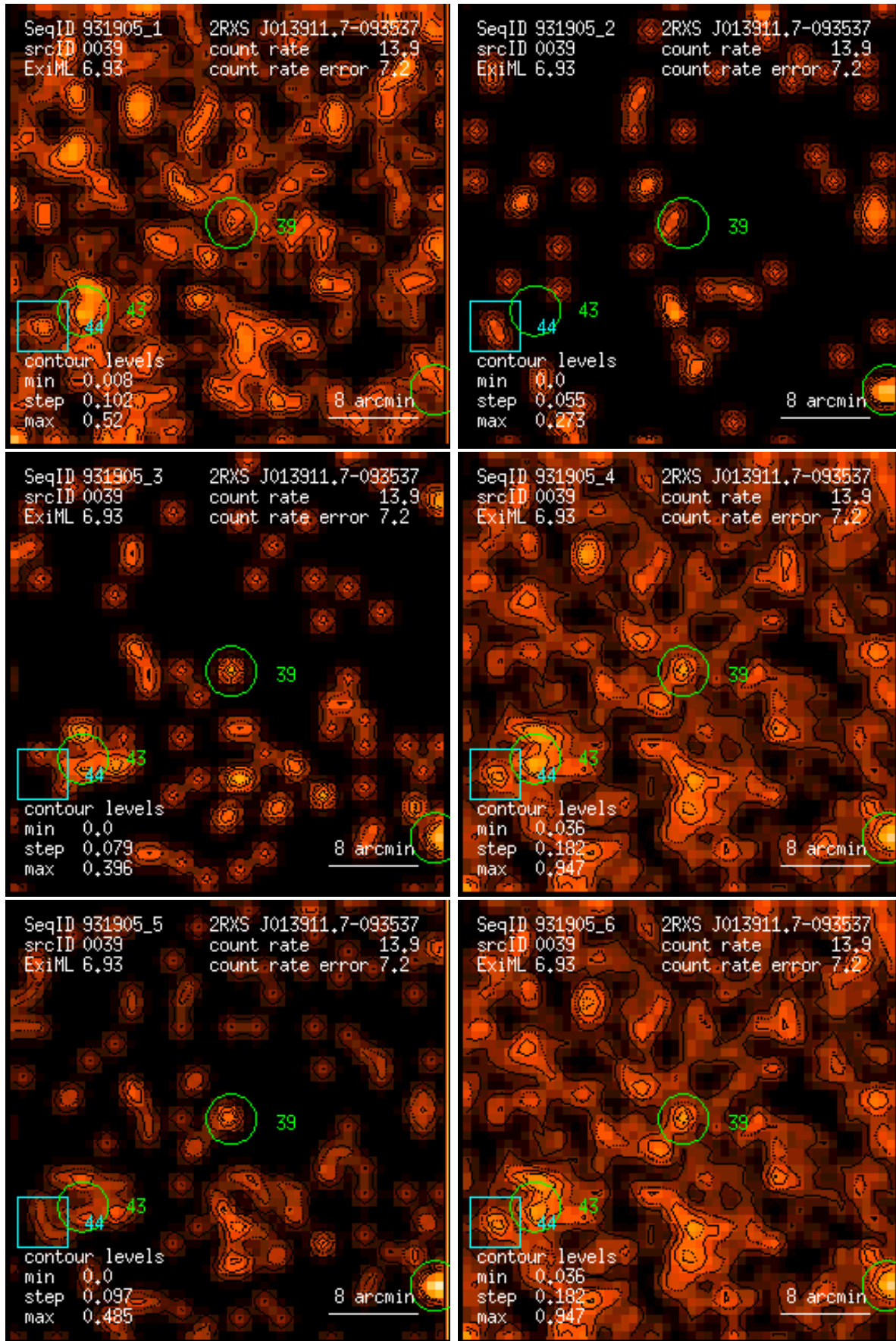
Figure 39: RASS 931905: detection 0039: band rate images, Gaussian filter: (1) PSPC channels 11 – 41, (2) 52 – 90, (3) 91 – 201, (4) 11 – 235, (5) 52 – 201, (6) 11 – 201. Broad band rates in counts/ks. Band rate contour levels in counts/ks/arcmin 2 .
