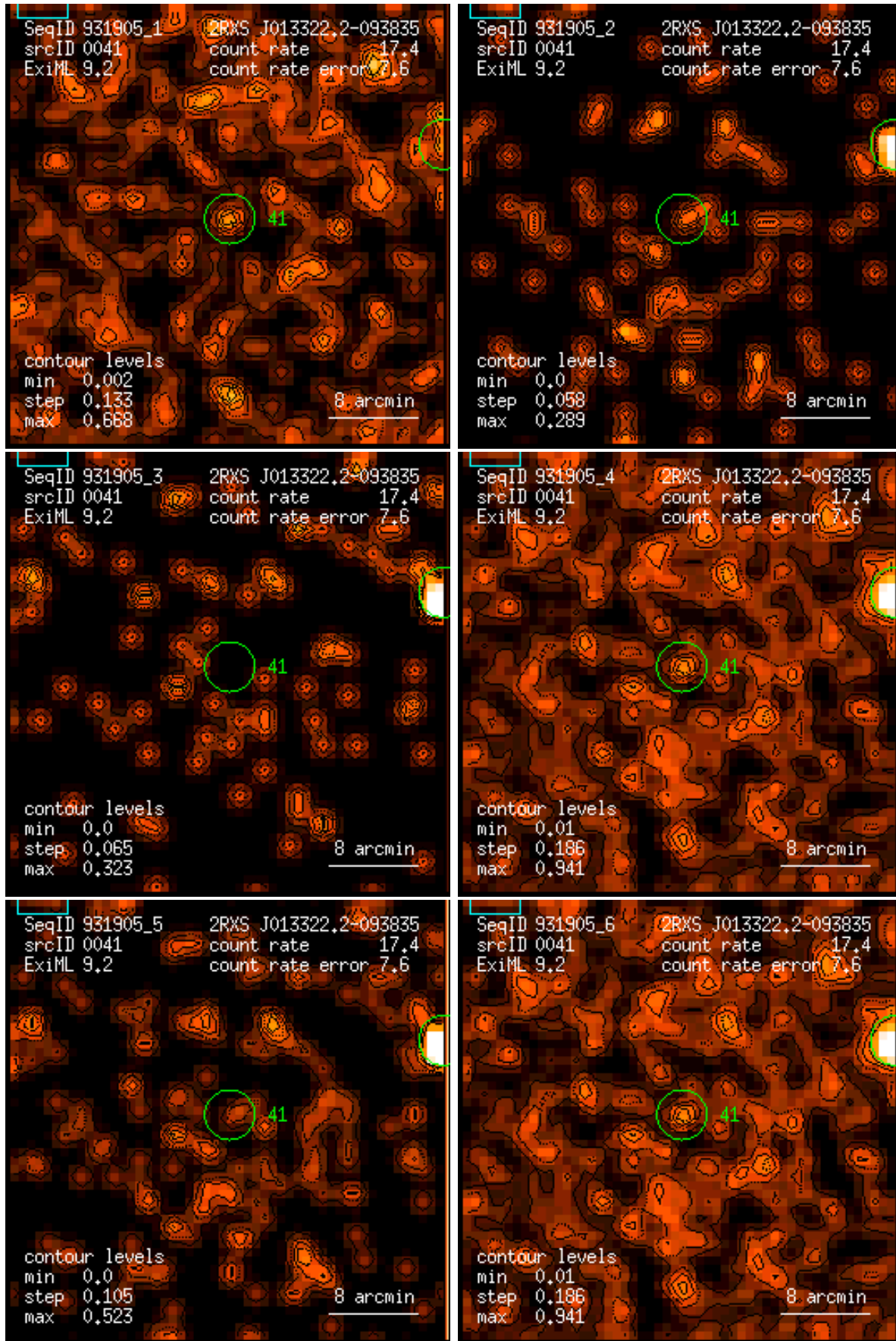
Figure 41: RASS 931905: detection 0041: band rate images, Gaussian filter: (1) PSPC channels 11 – 41, (2) 52 – 90, (3) 91 – 201, (4) 11 – 235, (5) 52 – 201, (6) 11 – 201. Broad band rates in counts/ks. Band rate contour levels in counts/ks/arcmin 2 .
