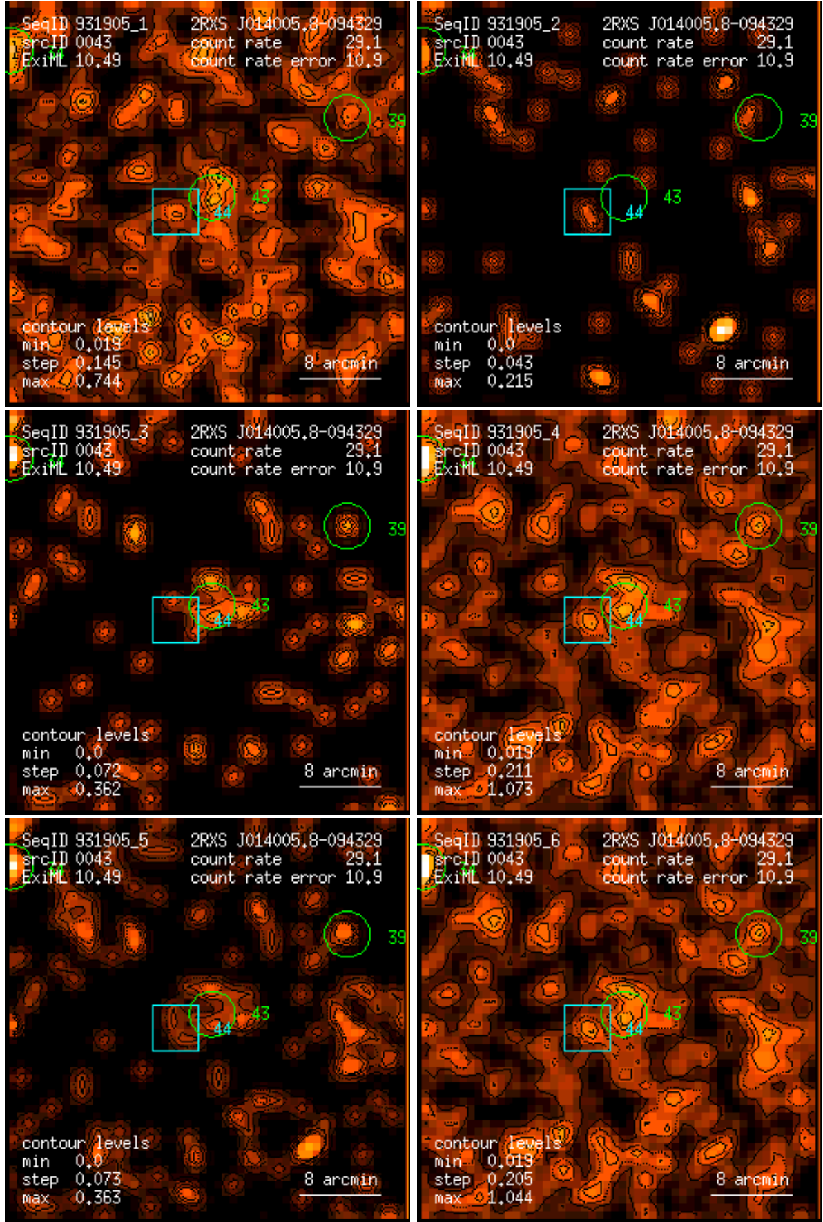
Figure 43: RASS 931905: detection 0043: band rate images, Gaussian filter: (1) PSPC channels 11 – 41, (2) 52 – 90, (3) 91 – 201, (4) 11 – 235, (5) 52 – 201, (6) 11 – 201. Broad band rates in counts/ks. Band rate contour levels in counts/ks/arcmin 2 .
