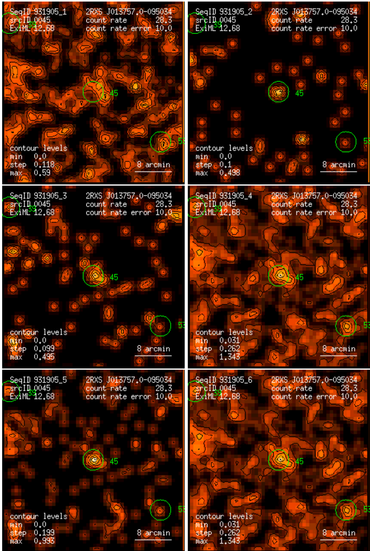
Figure 45: RASS 931905: detection 0045: band rate images, Gaussian filter: (1) PSPC channels 11 – 41, (2) 52 – 90, (3) 91 – 201, (4) 11 – 235, (5) 52 – 201, (6) 11 – 201. Broad band rates in counts/ks. Band rate contour levels in counts/ks/arcmin 2 .
