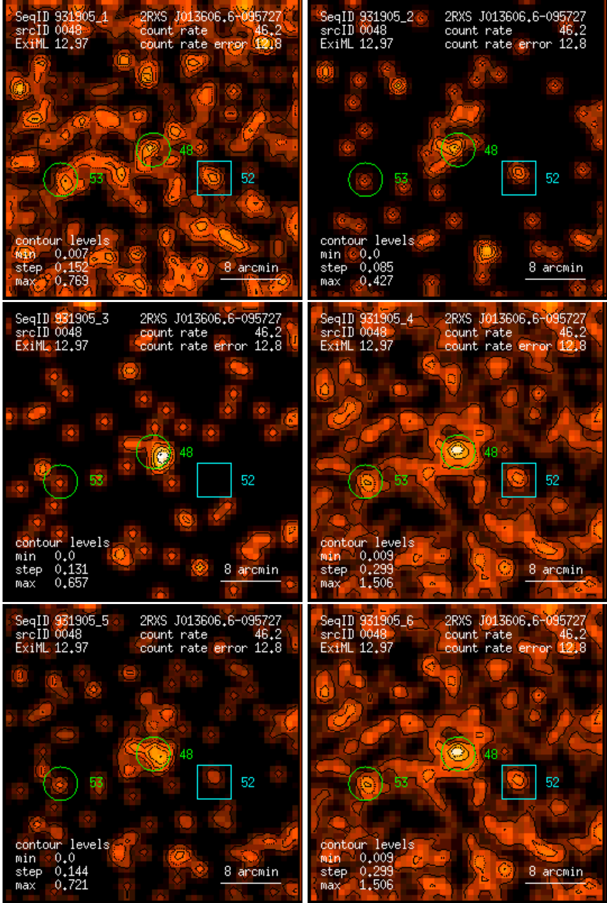
Figure 48: RASS 931905: detection 0048: band rate images, Gaussian filter: (1) PSPC channels 11 – 41, (2) 52 – 90, (3) 91 – 201, (4) 11 – 235, (5) 52 – 201, (6) 11 – 201. Broad band rates in counts/ks. Band rate contour levels in counts/ks/arcmin 2 .
