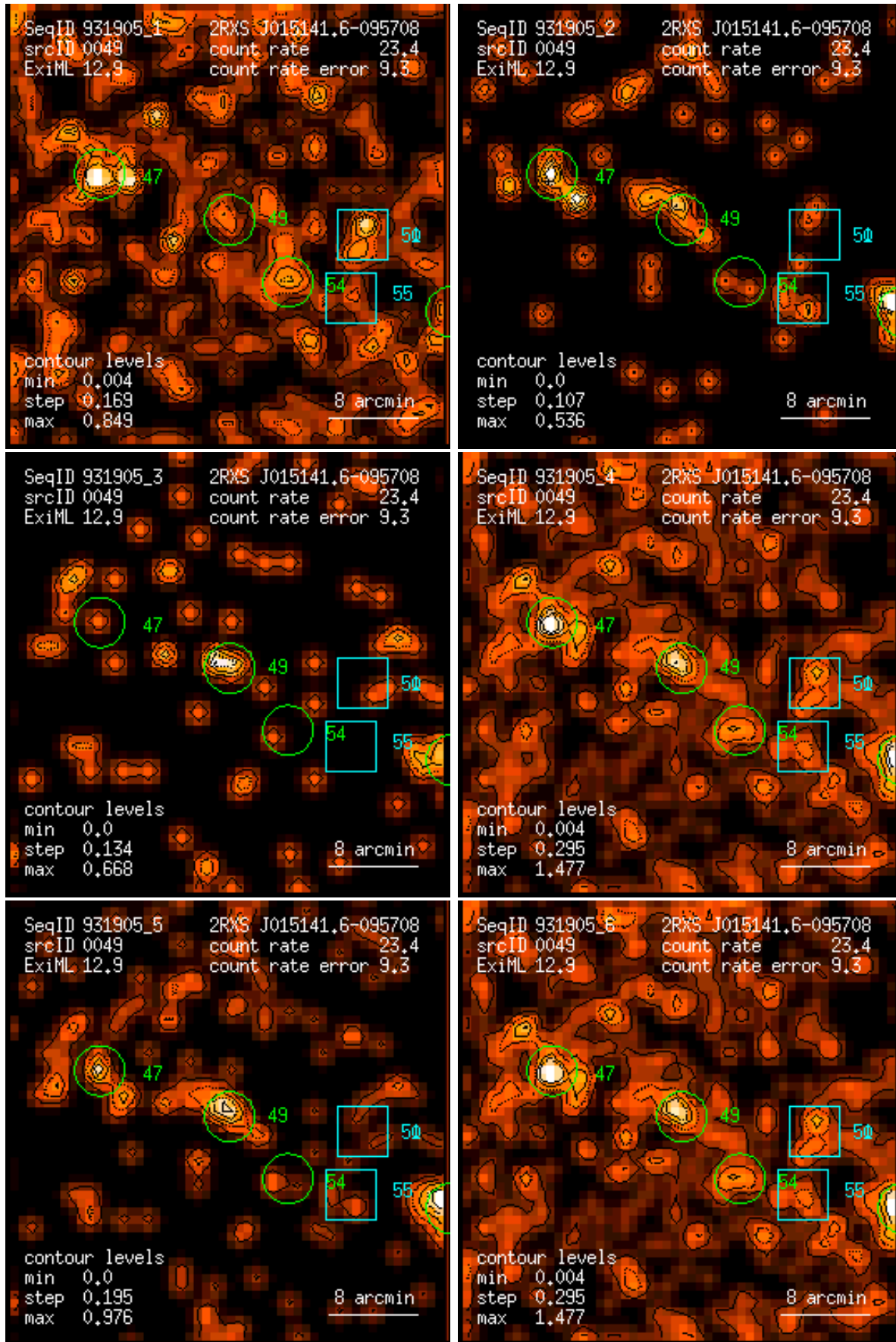
Figure 49: RASS 931905: detection 0049: band rate images, Gaussian filter: (1) PSPC channels 11 – 41, (2) 52 – 90, (3) 91 – 201, (4) 11 – 235, (5) 52 – 201, (6) 11 – 201. Broad band rates in counts/ks. Band rate contour levels in counts/ks/arcmin 2 .
