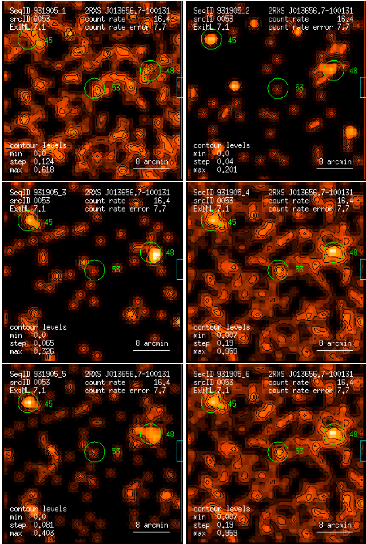
Figure 53: RASS 931905: detection 0053: band rate images, Gaussian filter: (1) PSPC channels 11 – 41, (2) 52 – 90, (3) 91 – 201, (4) 11 – 235, (5) 52 – 201, (6) 11 – 201. Broad band rates in counts/ks. Band rate contour levels in counts/ks/arcmin 2 .
