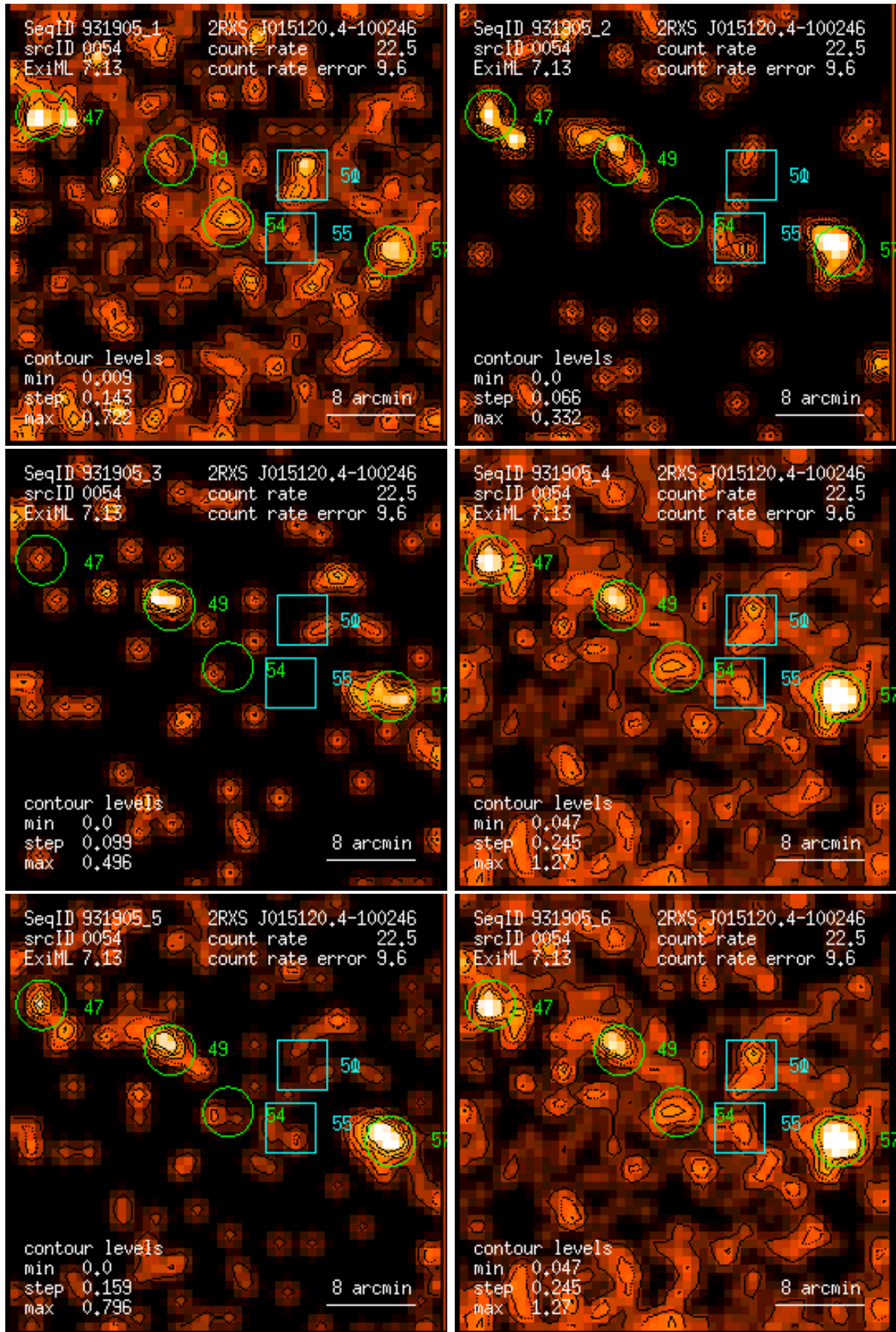
Figure 54: RASS 931905: detection 0054: band rate images, Gaussian filter: (1) PSPC channels 11 – 41, (2) 52 – 90, (3) 91 – 201, (4) 11 – 235, (5) 52 – 201, (6) 11 – 201. Broad band rates in counts/ks. Band rate contour levels in counts/ks/arcmin 2 .
