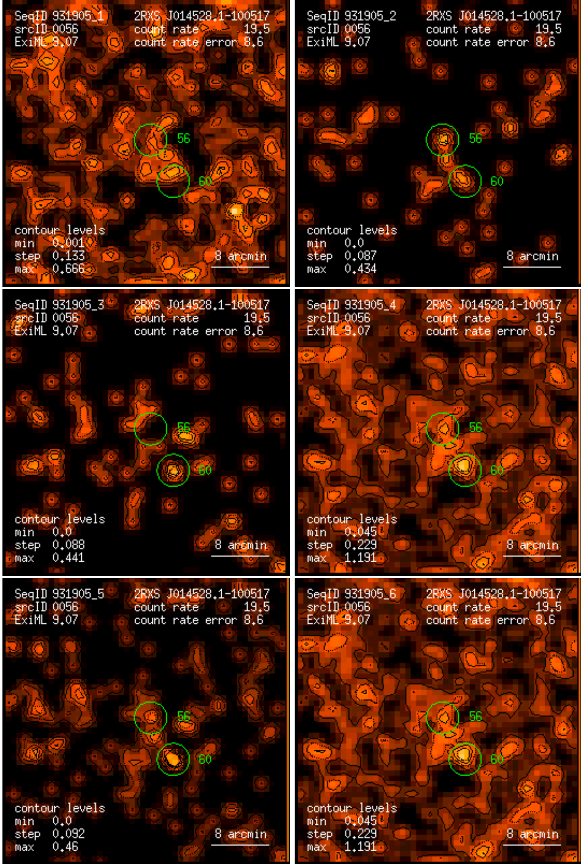
Figure 56: RASS 931905: detection 0056: band rate images, Gaussian filter: (1) PSPC channels 11 – 41, (2) 52 – 90, (3) 91 – 201, (4) 11 – 235, (5) 52 – 201, (6) 11 – 201. Broad band rates in counts/ks. Band rate contour levels in counts/ks/arcmin 2 .
