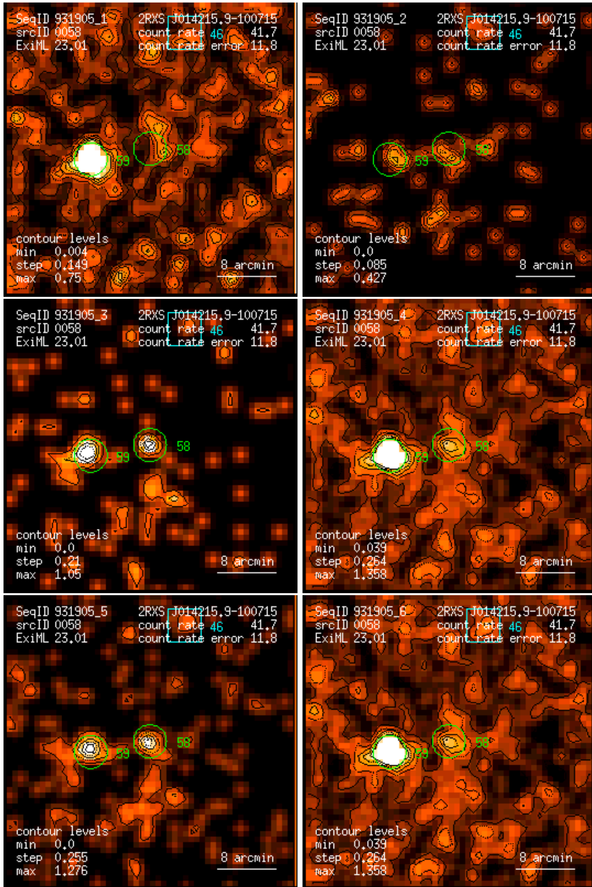
Figure 58: RASS 931905: detection 0058: band rate images, Gaussian filter: (1) PSPC channels 11 – 41, (2) 52 – 90, (3) 91 – 201, (4) 11 – 235, (5) 52 – 201, (6) 11 – 201. Broad band rates in counts/ks. Band rate contour levels in counts/ks/arcmin 2 .
