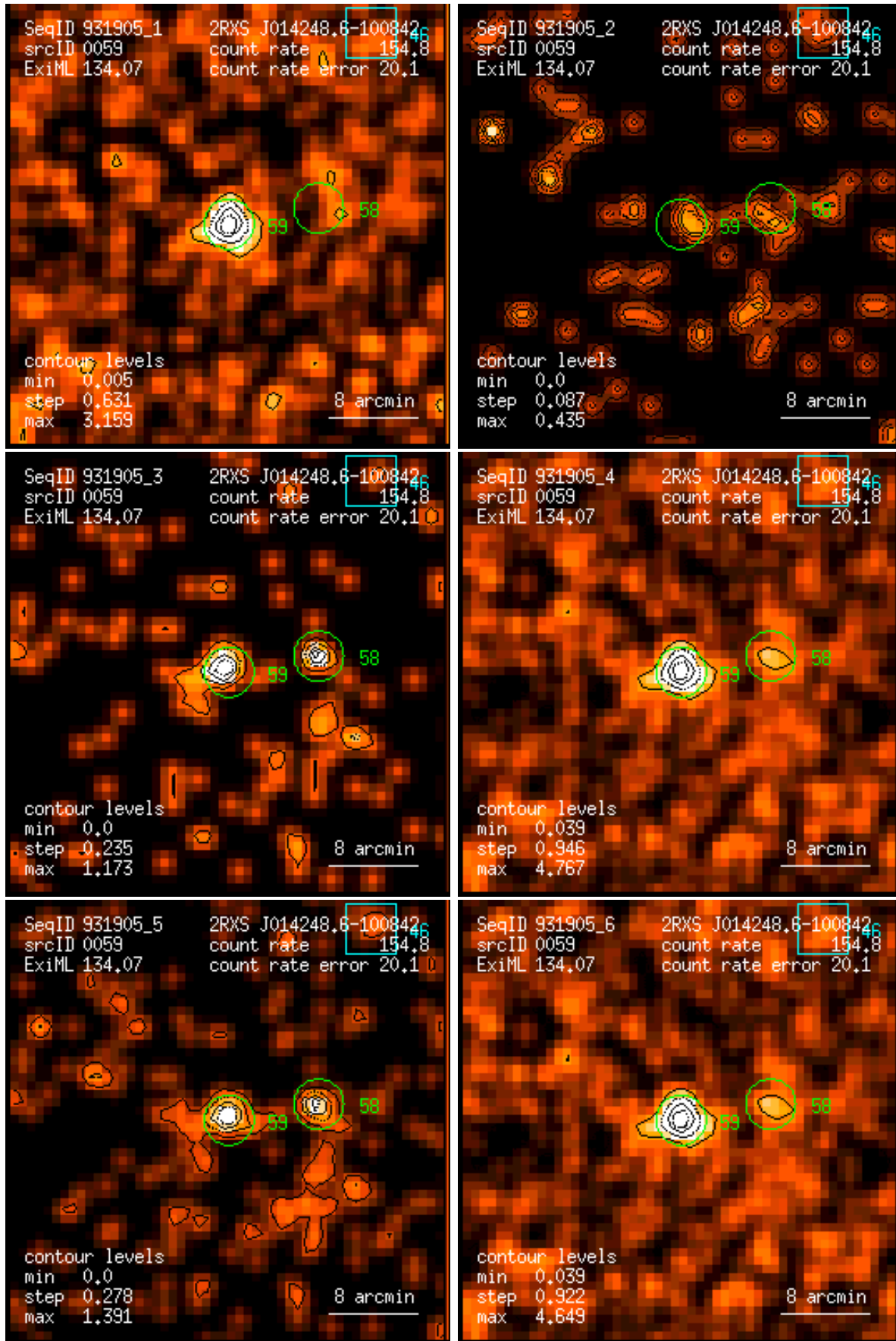
Figure 59: RASS 931905: detection 0059: band rate images, Gaussian filter: (1) PSPC channels 11 – 41, (2) 52 – 90, (3) 91 – 201, (4) 11 – 235, (5) 52 – 201, (6) 11 – 201. Broad band rates in counts/ks. Band rate contour levels in counts/ks/arcmin 2 .
