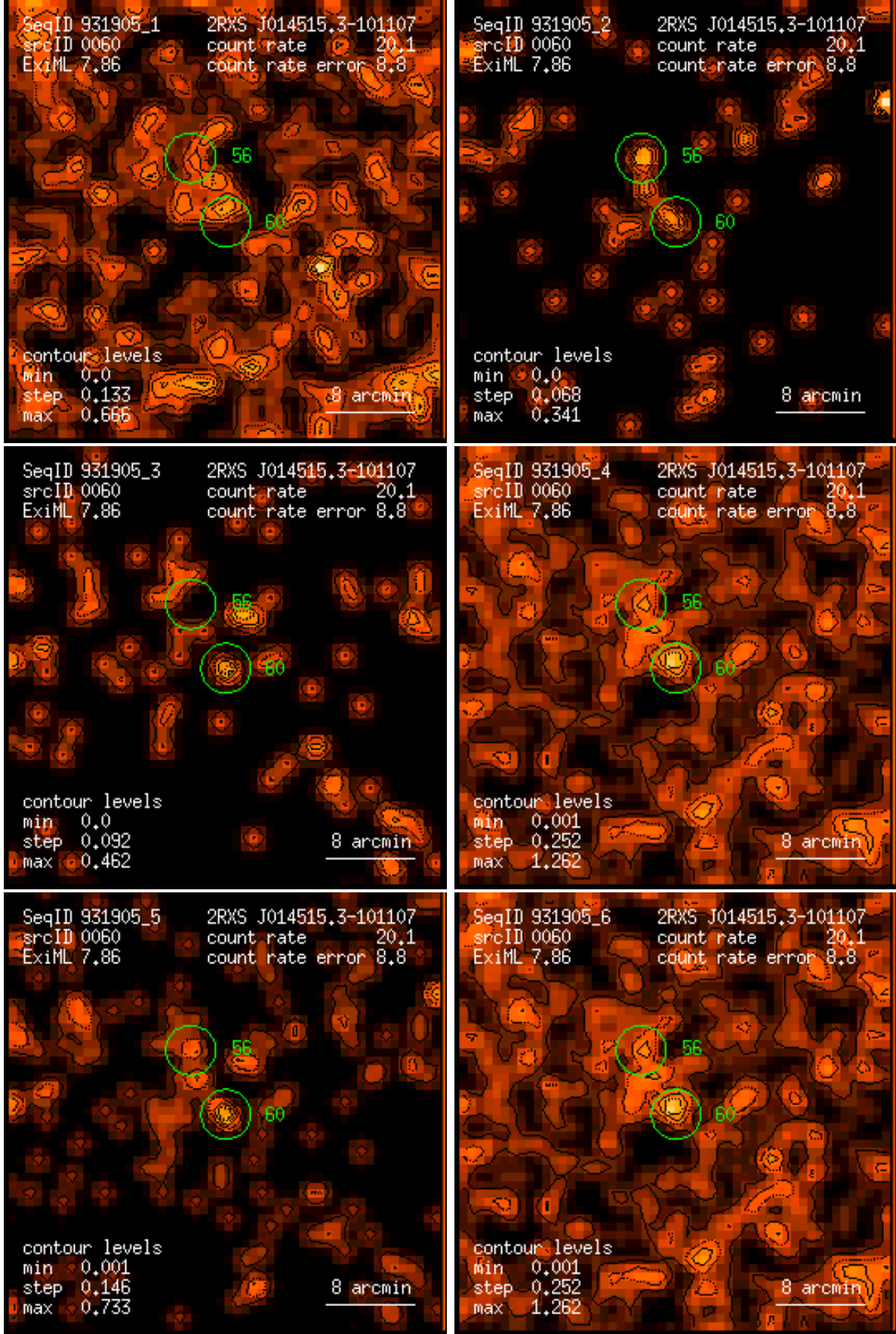
Figure 60: RASS 931905: detection 0060: band rate images, Gaussian filter: (1) PSPC channels 11 – 41, (2) 52 – 90, (3) 91 – 201, (4) 11 – 235, (5) 52 – 201, (6) 11 – 201. Broad band rates in counts/ks. Band rate contour levels in counts/ks/arcmin 2 .
